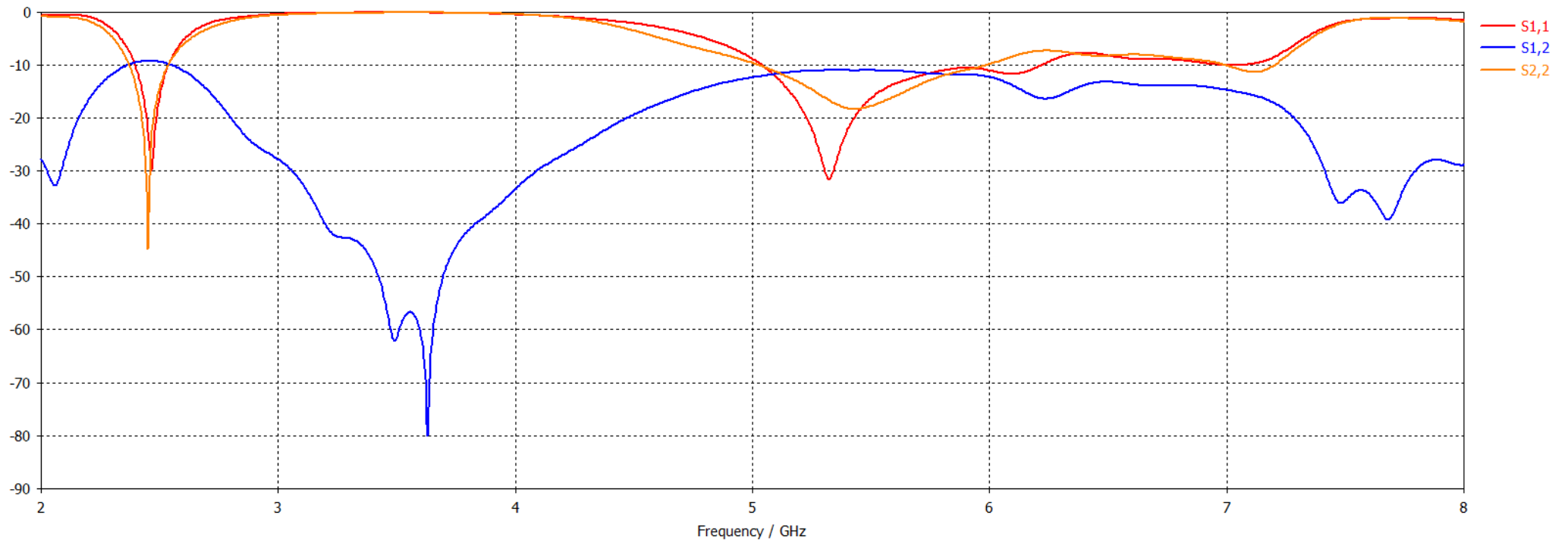
S-Parameter [Magnitude in dB]
