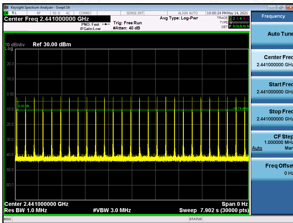
BR_HOP_ANT1_NA_1Mbps_2441_Number of Burst
