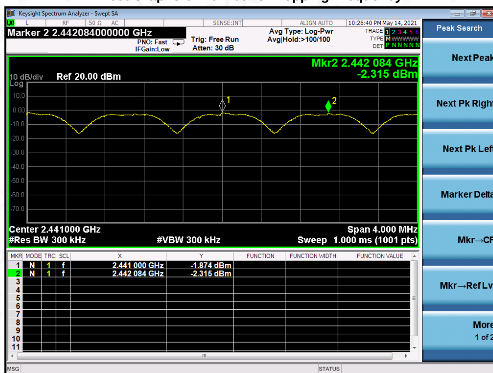
BR_HOP_ANT1_NA_1Mbps_Hopping Separation
