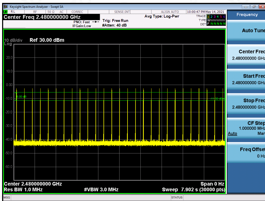
BR_HOP_ANT1_NA_1Mbps_2480_Number of Burst
