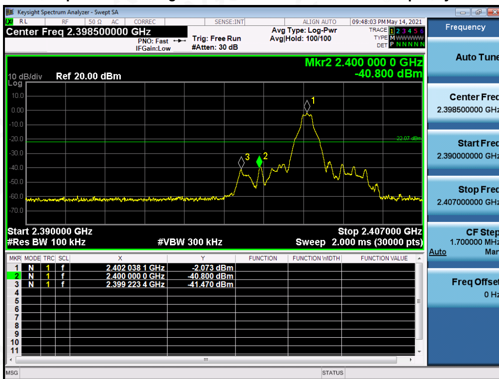
BR_ANT1_2402_1Mbps_Lower Band Edge Emissions
