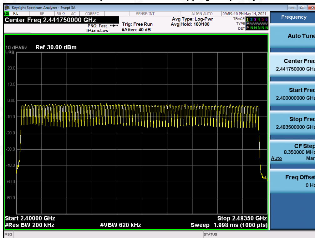
BR_HOP_ANT1_NA_1Mbps_Number of Hopping
