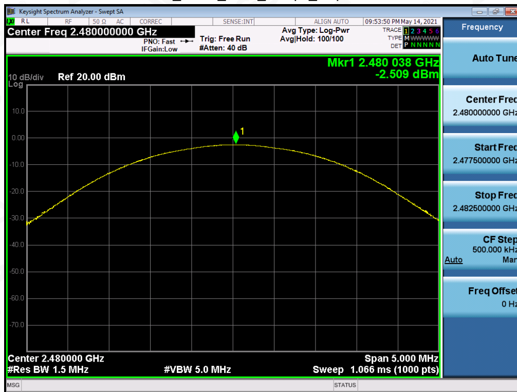
BR_ANT1_2480_1Mbps_PKpower
