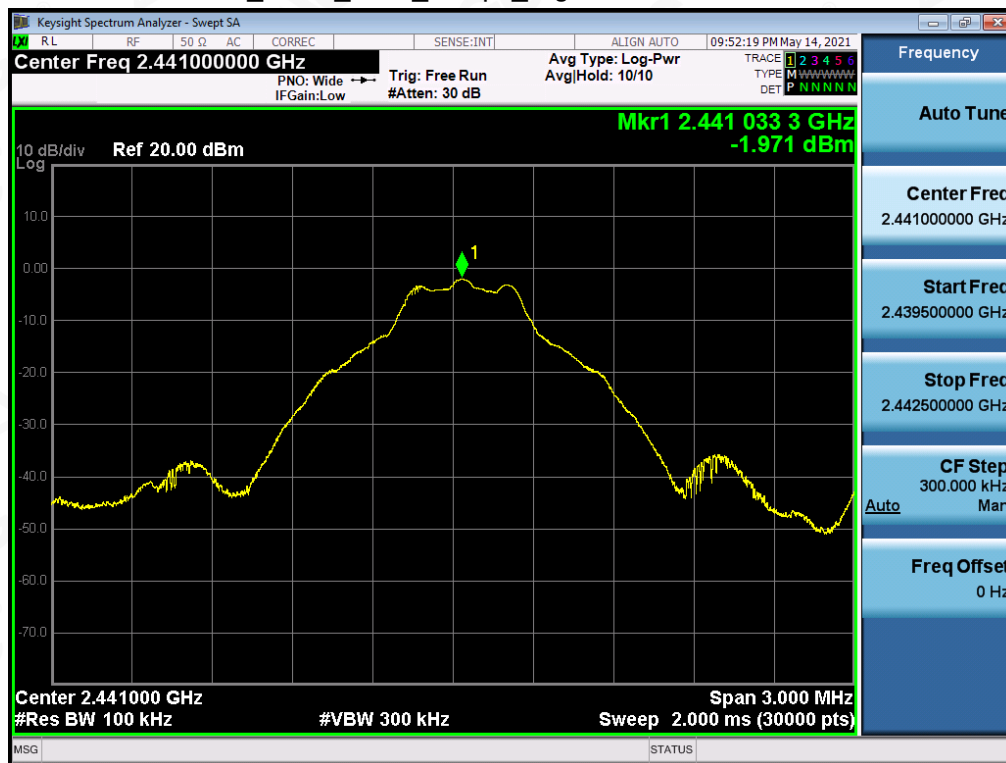
BR_ANT1_2441_1Mbps_Reference Level
