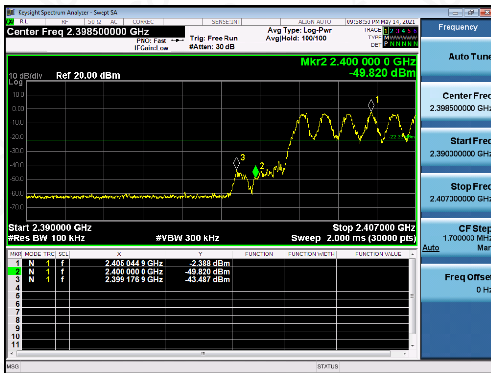
BR_HOP_ANT1_NA_1Mbps_Lower Band Edge Emissions
