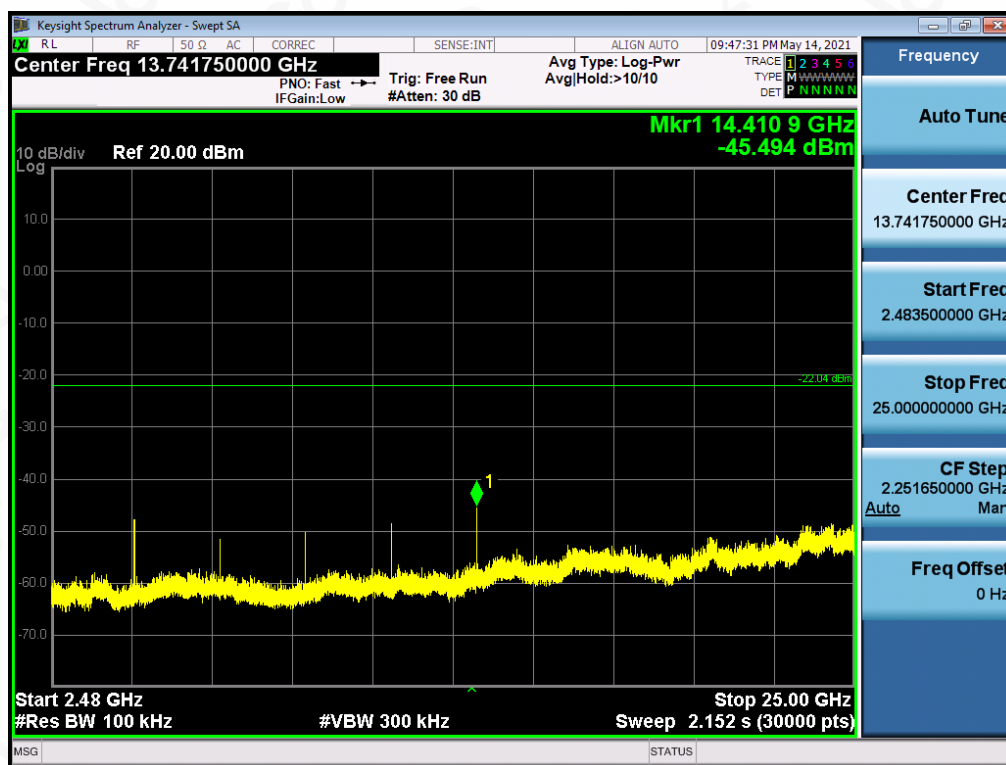
BR_ANT1_2402_1Mbps_Higher Band Emissions
