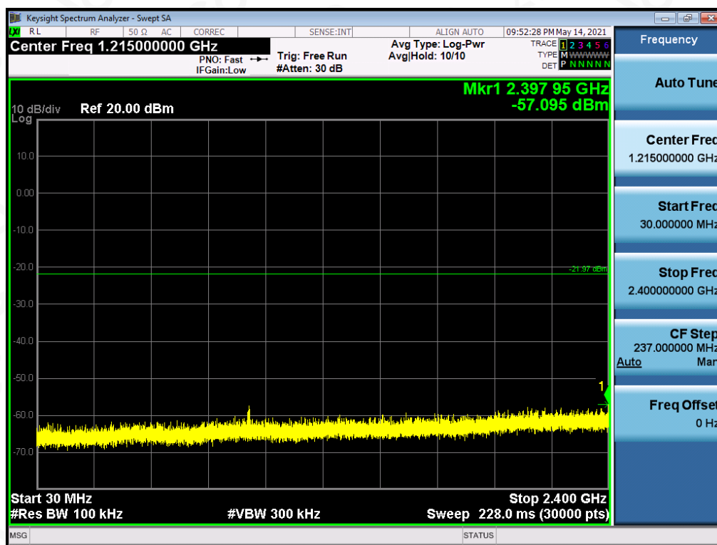
BR_ANT1_2441_1Mbps_Lower Band Emissions
