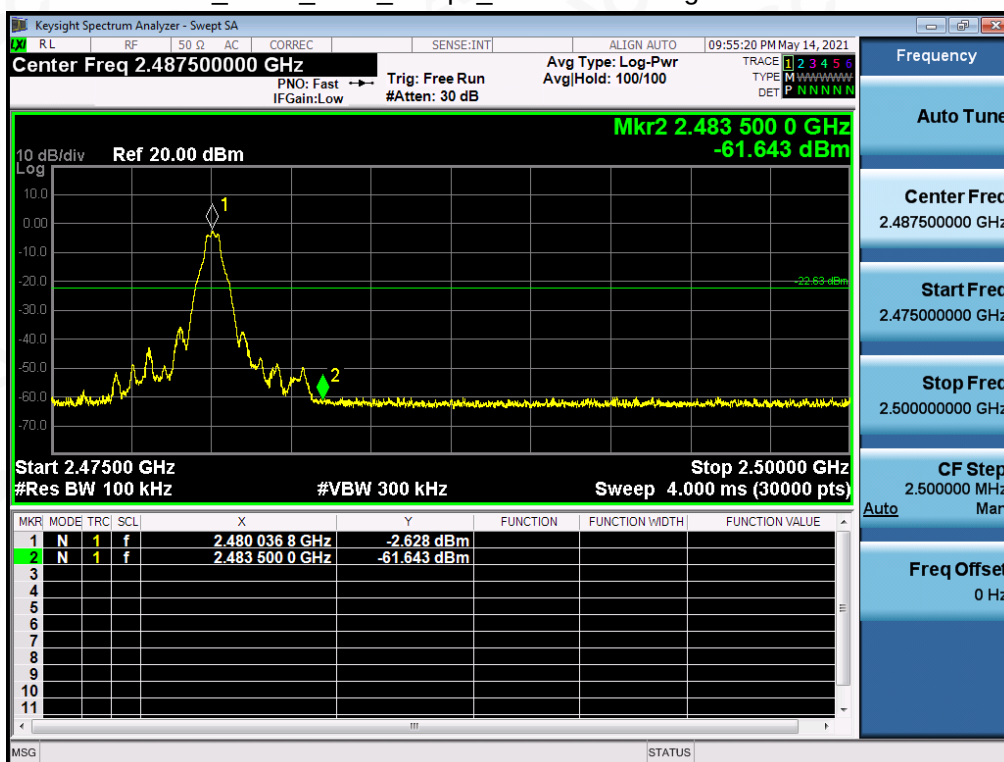
BR_ANT1_2480_1Mbps_Higher Band Edge Emissions
