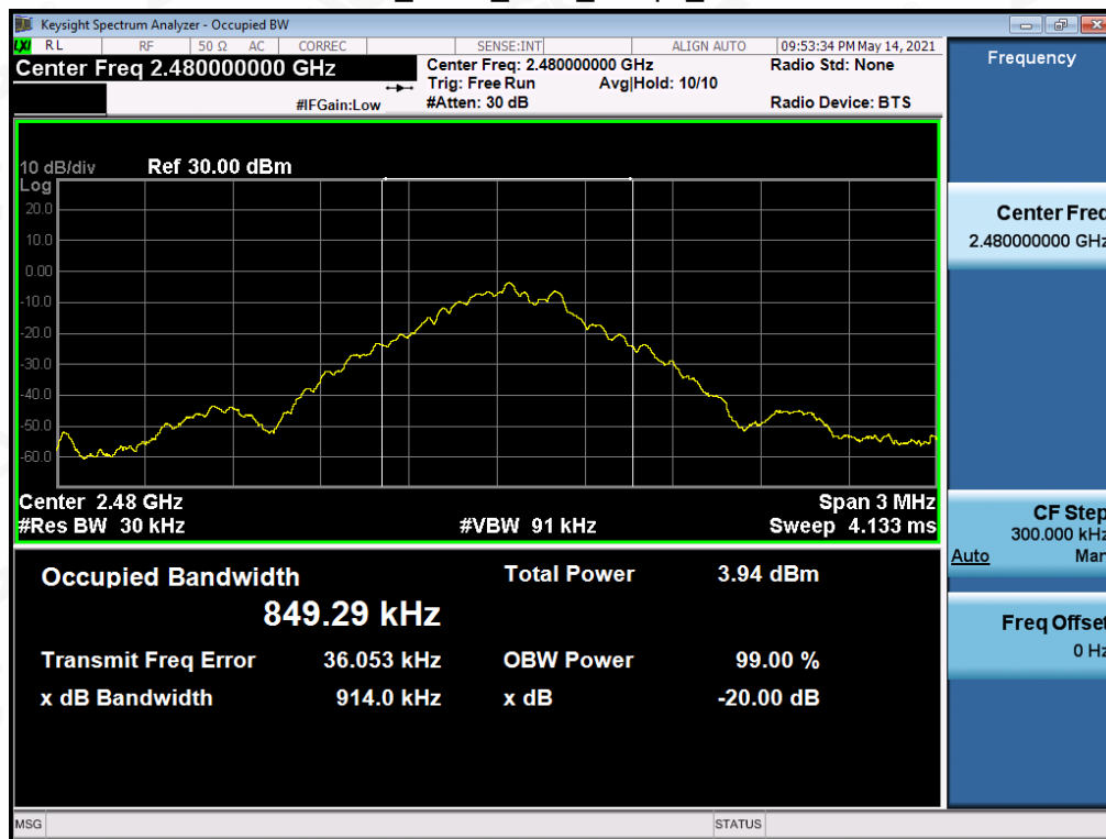
BR_ANT1_2480_1Mbps_OBW
