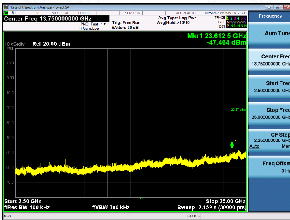
BR_ANT1_2480_1Mbps_Higher Band Emissions
