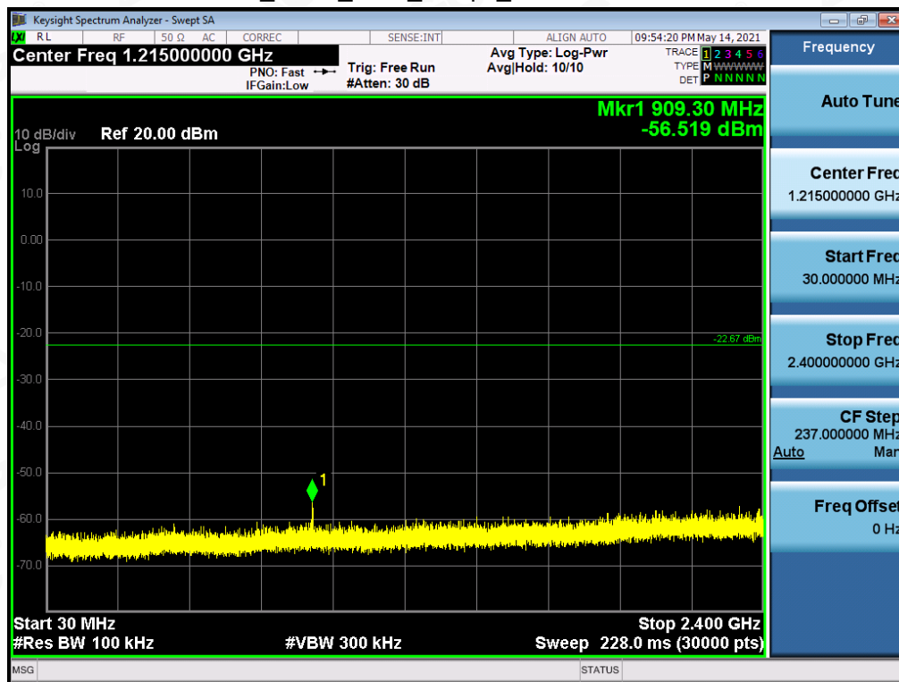
BR_ANT1_2480_1Mbps_Lower Band Emissions
