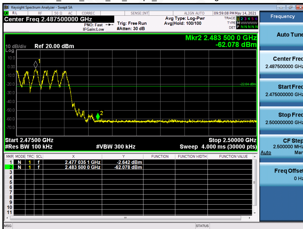
BR_HOP_ANT1_NA_1Mbps_Higher Band Edge Emissions
