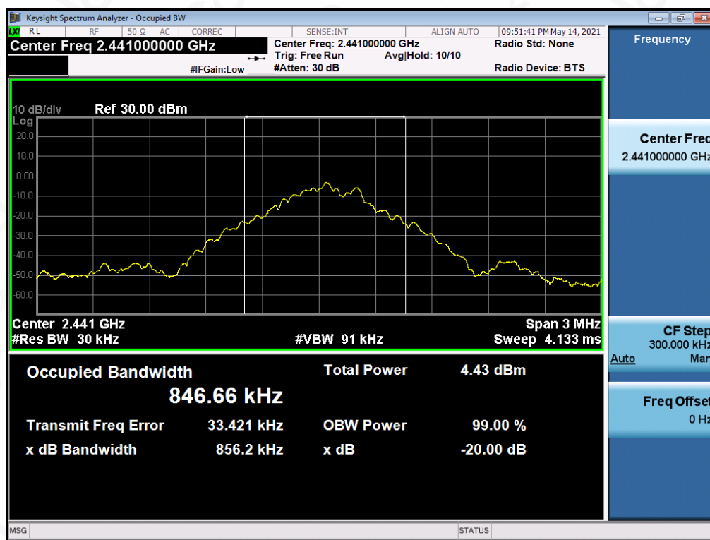
BR_ANT1_2441_1Mbps_OBW
