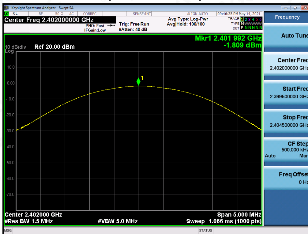
BR_ANT1_2402_1Mbps_PKpower
