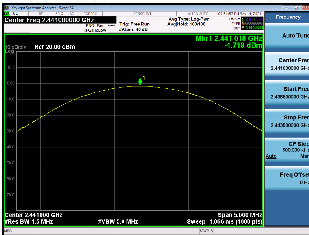
BR_ANT1_2441_1Mbps_PKpower
