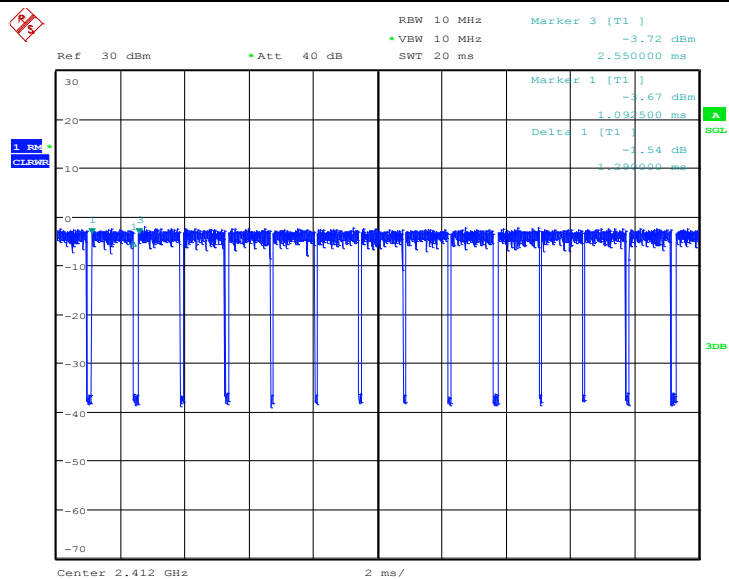
Test Graph_ IEEE802.11 n (HT20) Duty Cycle: 88.51%
