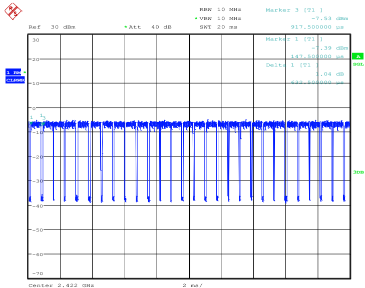
Test Graph_ IEEE802.11 n (HT40) Duty Cycle: 82.14%
