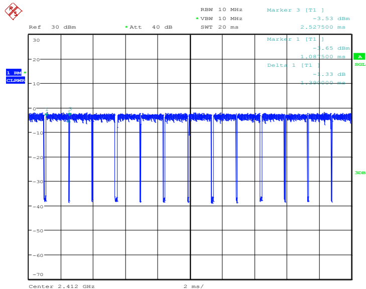
Test Graph_ IEEE802.11g Duty Cycle: 96.53%
