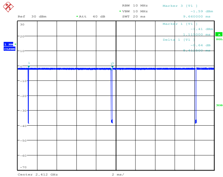
Test Graph_ IEEE802.11b Duty Cycle: 98.45%
