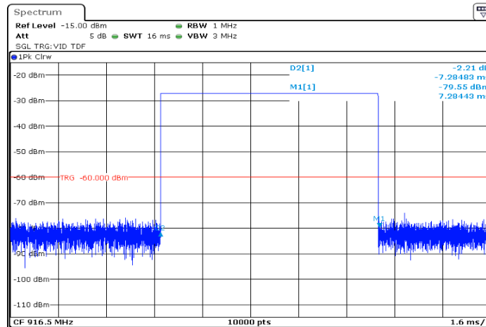
Plot 7.2.7 Transmission pulse duration
