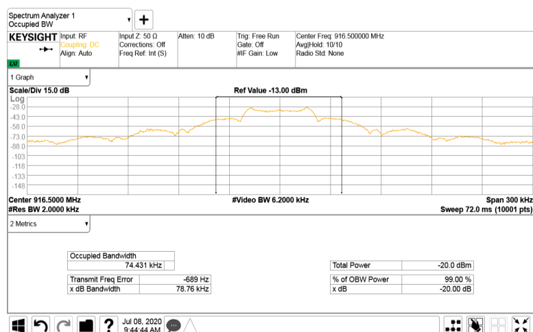
Plot 7.3.1 Occupied bandwidth test results
