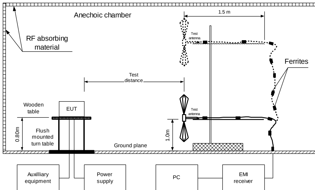
Figure 8.2.1 Setup for radiated emission measurements
