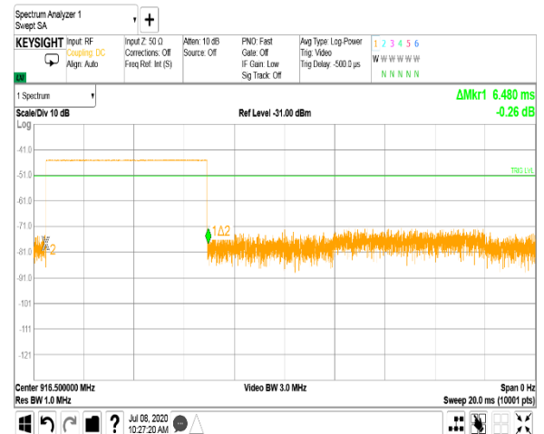
Plot 7.1.2 Polling / supervision transmission duration
