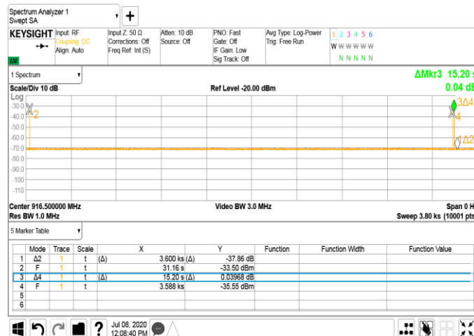
Plot 7.1.2 Polling / supervision transmission duration
