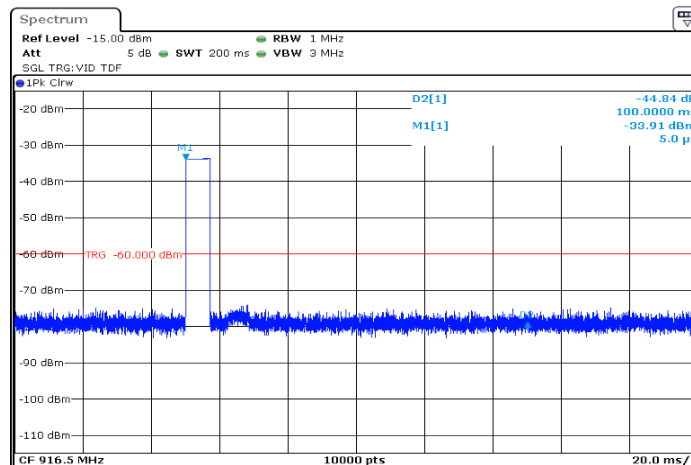
Plot 7.2.8 Transmission pulse period
