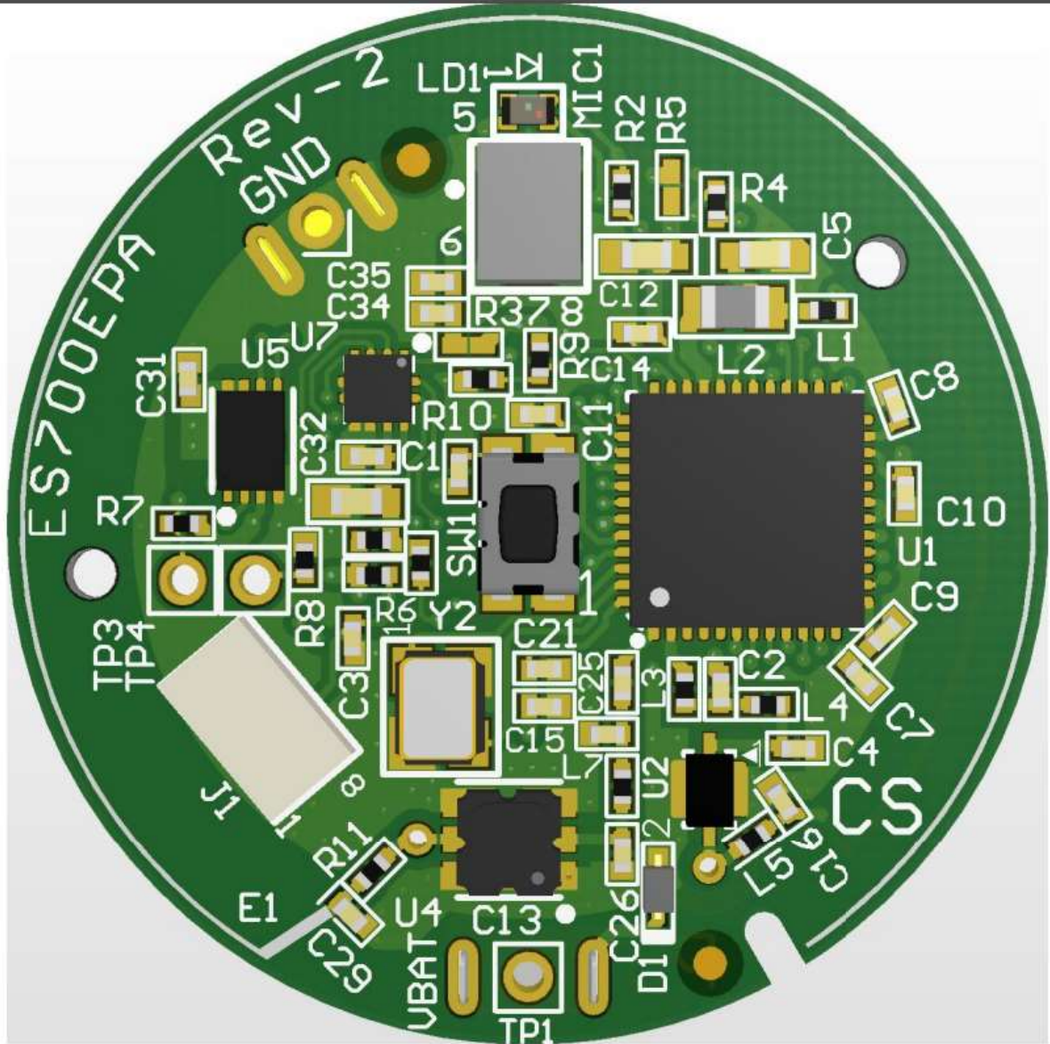
E1: Printed Antenna 916.5MHz; Gain -8.2dBm
