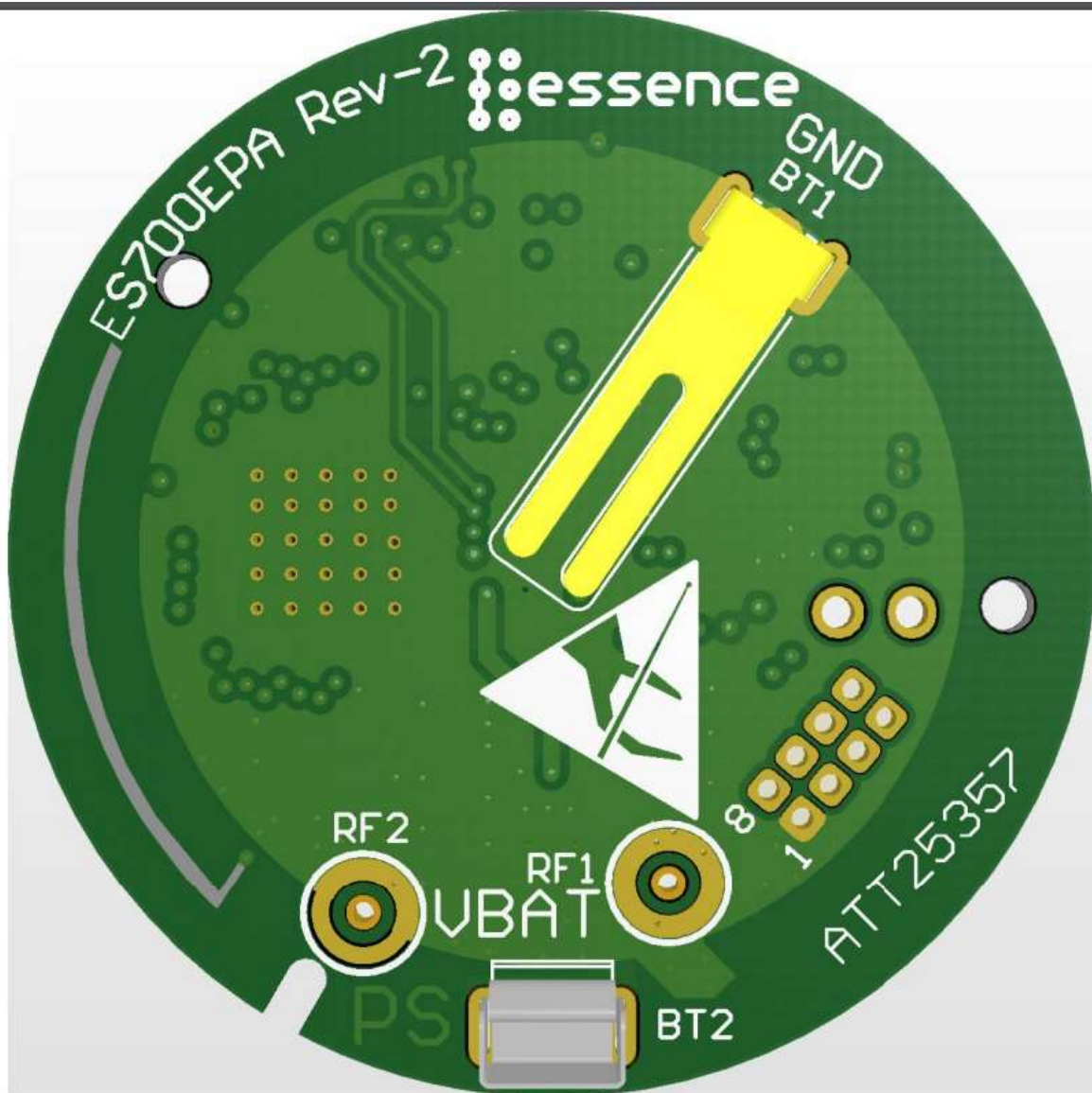
E2: Printed Antenna BLE 2.4GHz; Gain -3dBm
