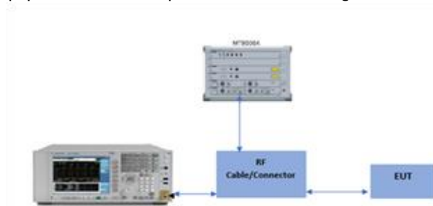
Figure 7-3. Test Instrument & Measurement Setup
