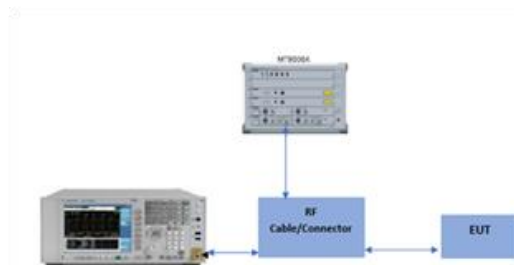
Figure 7-1. Test Instrument & Measurement Setup
