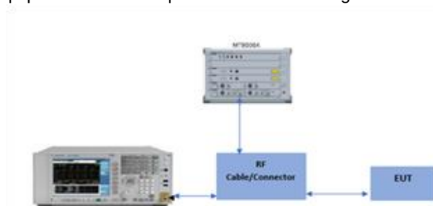
Figure 7-4. Test Instrument & Measurement Setup
