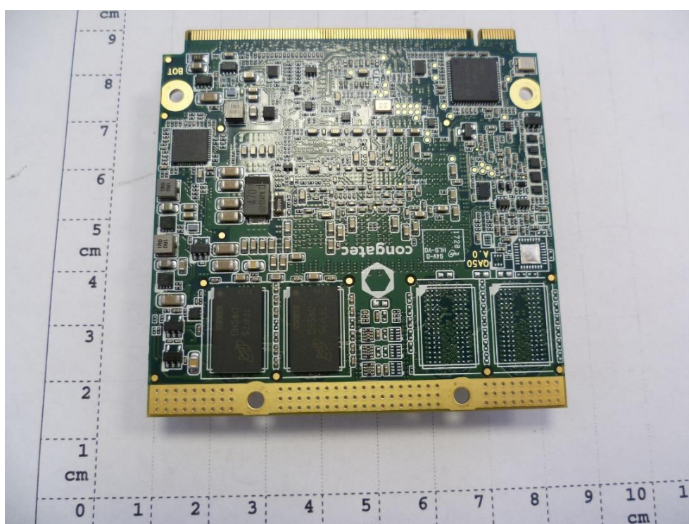
Figure 8: EUT digital pcb bottom view
