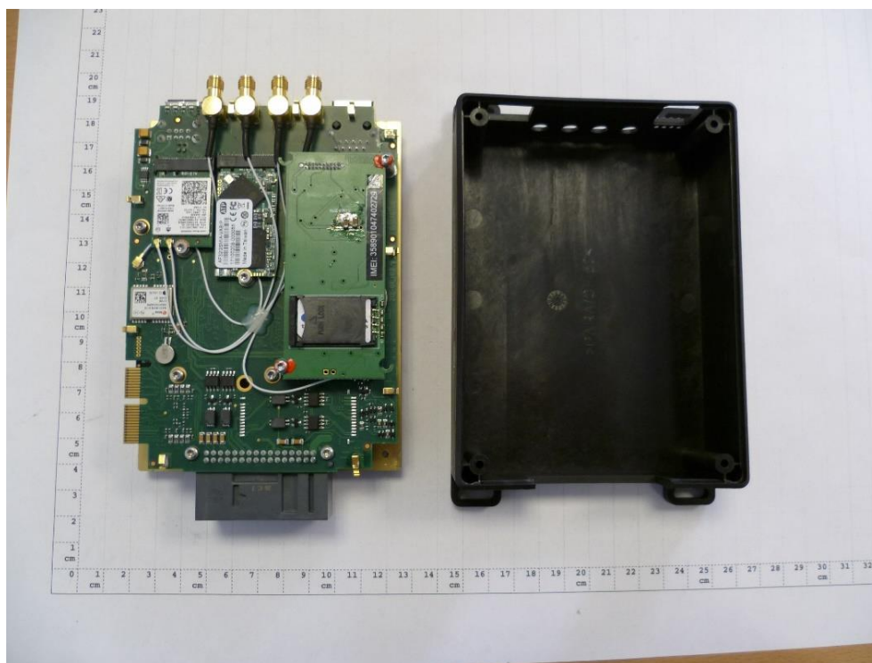
Figure 1: EUT inside view
