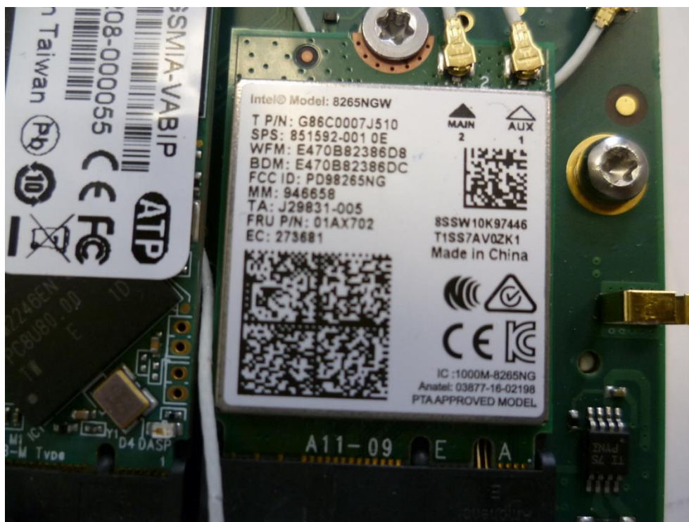
Figure 11: EUT WLAN and Bluetooth module
