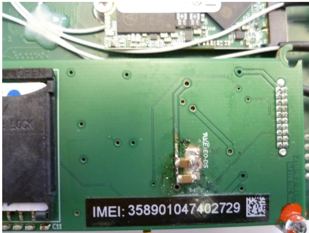
Figure 9: EUT modification to pass EMI AC
