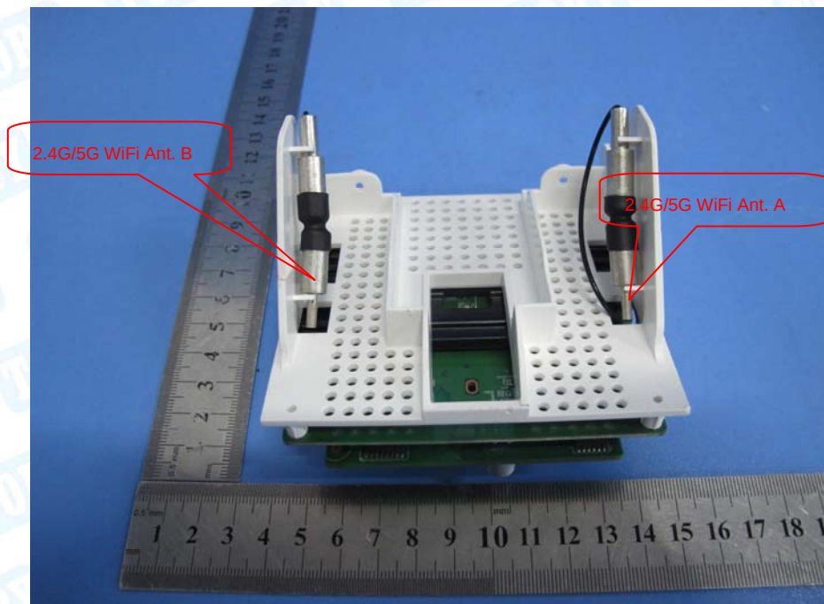
Photo 11 Internal of EUT
