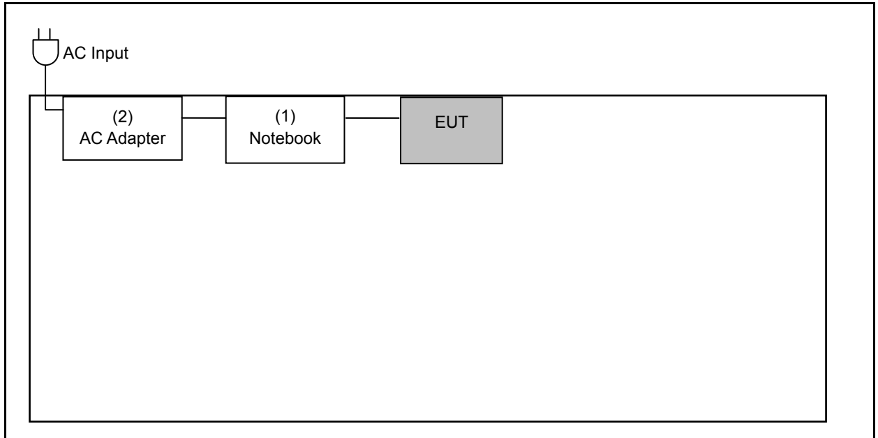
Conducted Emissions
