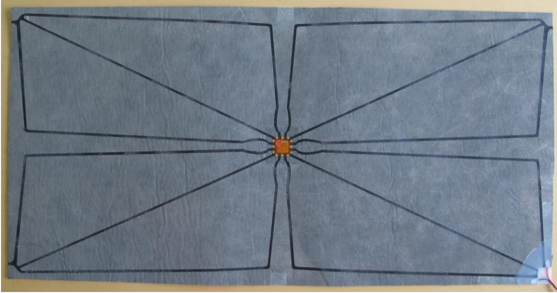
Sensor floor SF-LR (left), SF-HR (right)
