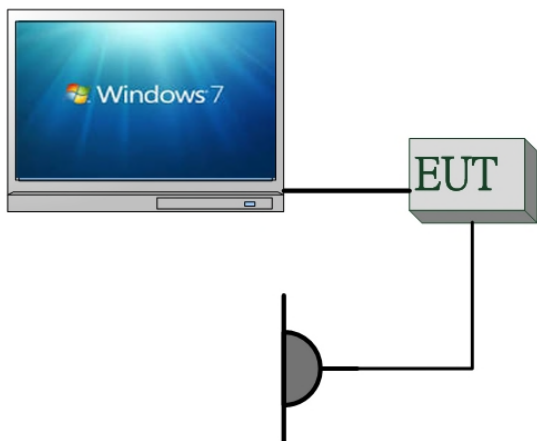
Fig. 2-1 Radiated Emission Configuration
