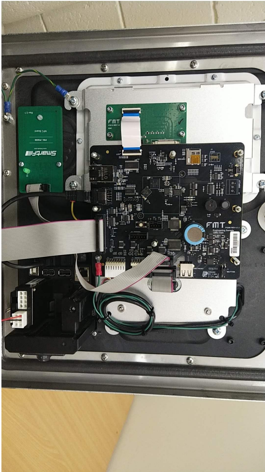
Panel board with shield board removed
