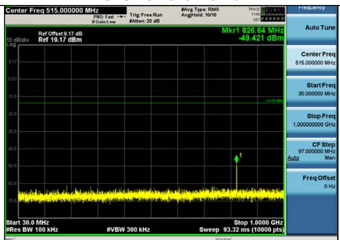
GFSK on Channel 78
