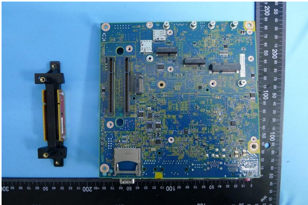
(56) Motherboard
