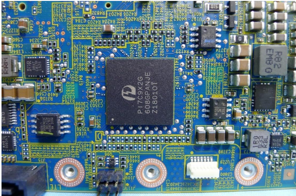
(54) Motherboard
