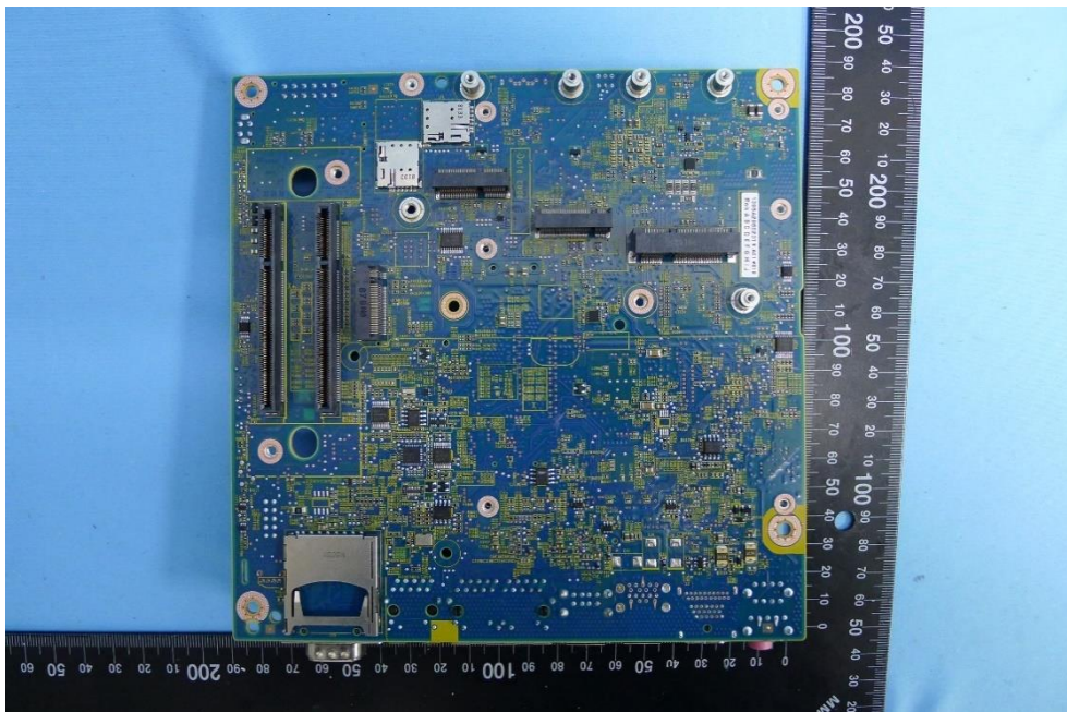
(56) Motherboard
