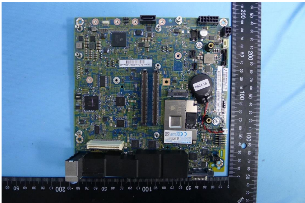
(48) Motherboard
