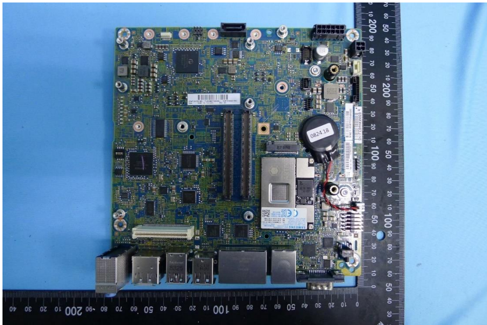
(50) Motherboard
