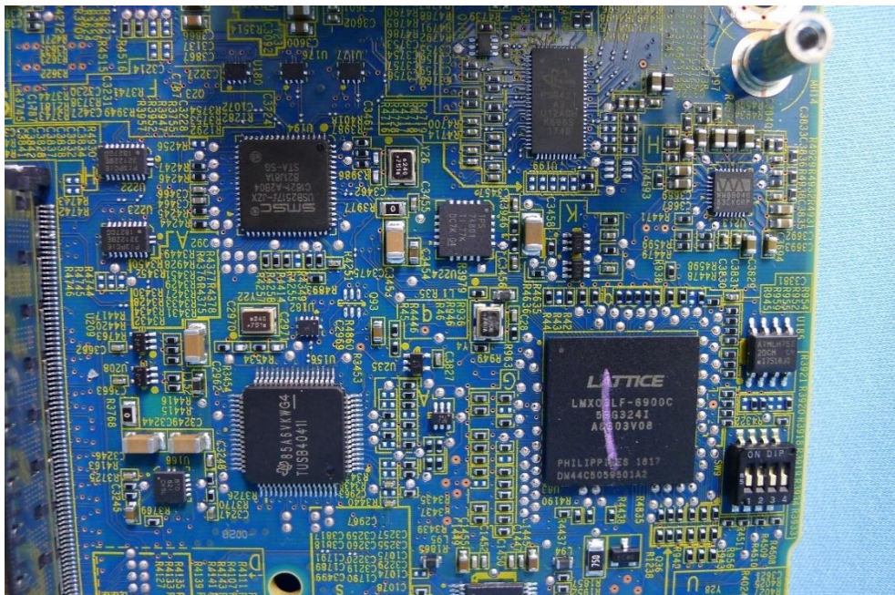
(52) Motherboard
