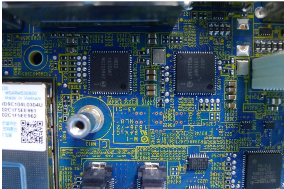
(52) Motherboard
