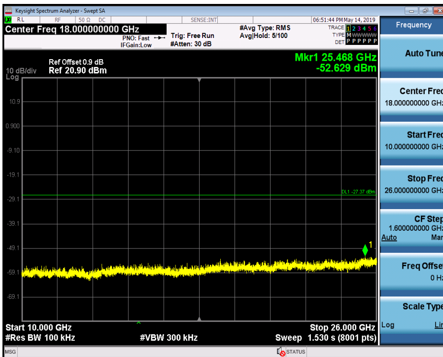
RF Conducted Spurious Emissions_BLE_2440_Ant1
