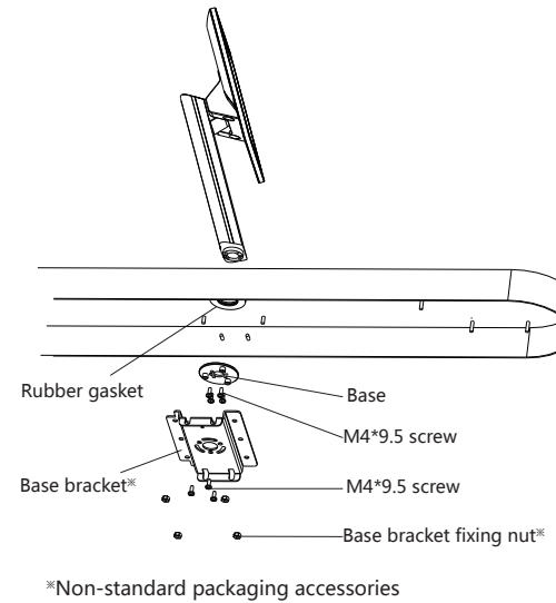
Installation diagram
