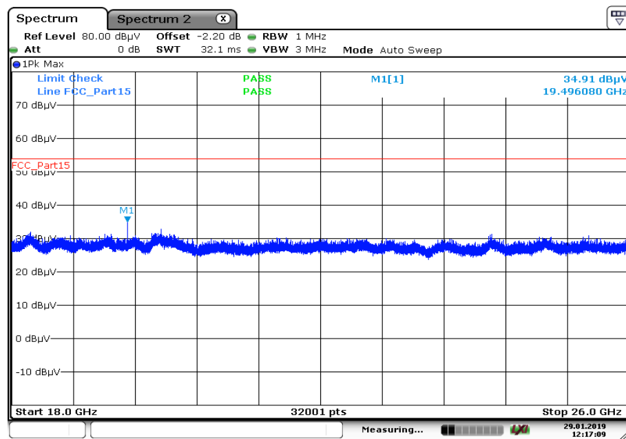
Plot 4: 18 GHz to 26 GHz, TX mode, 2441 MHz, vertical & horizontal polarization
