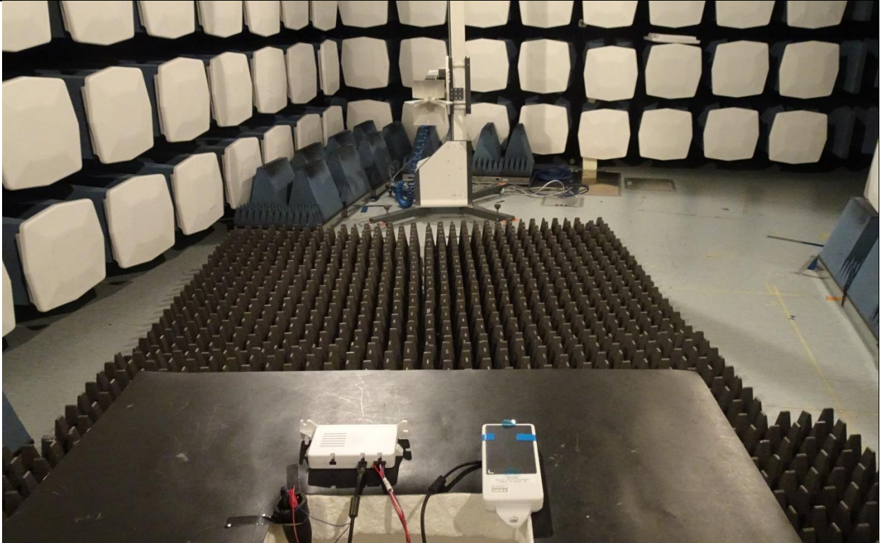
Picture 19, Radiated Spurious Emissions, common setup, RX, 1 – 18 GHz, back
