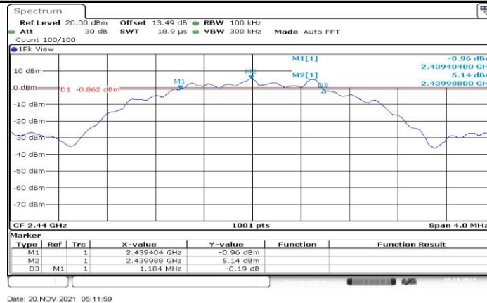
BLE_2M_Ant1_2440
