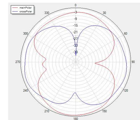
Theta=90 freq=5450MHz
