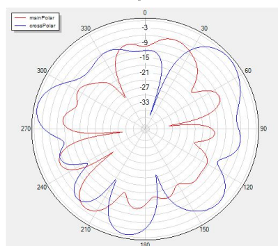
Phi=0 freq=2400MHz
