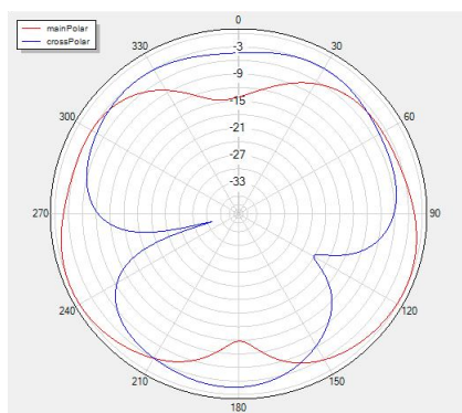
Theta=90 freq=2440MHz
