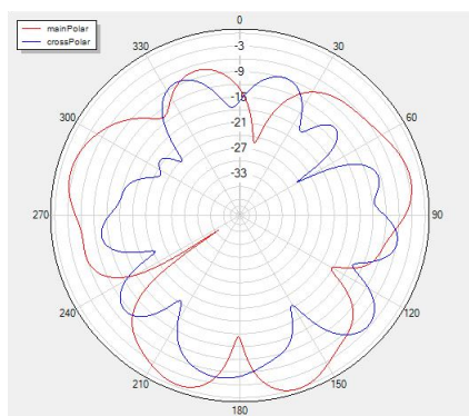
Phi=90 freq=2440MHz
