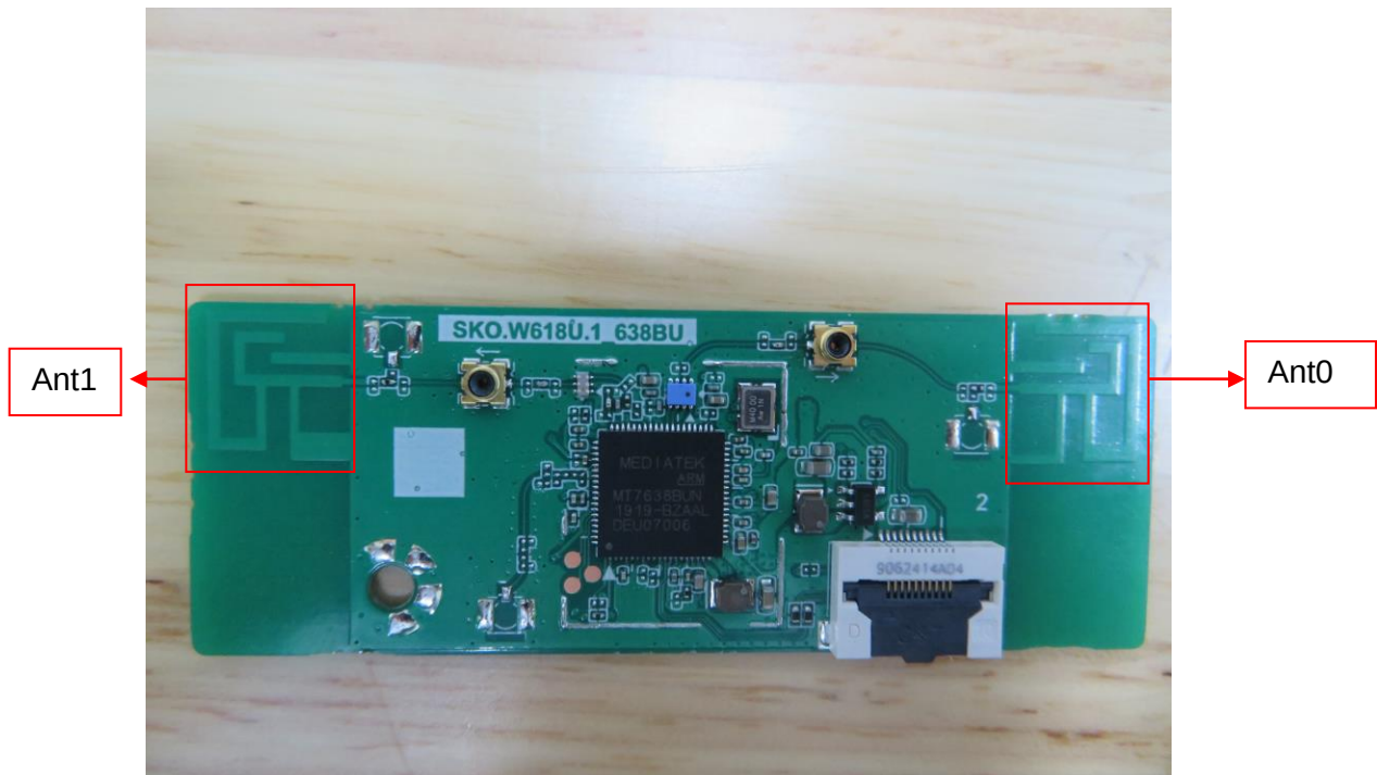
Open View of EUT-2
