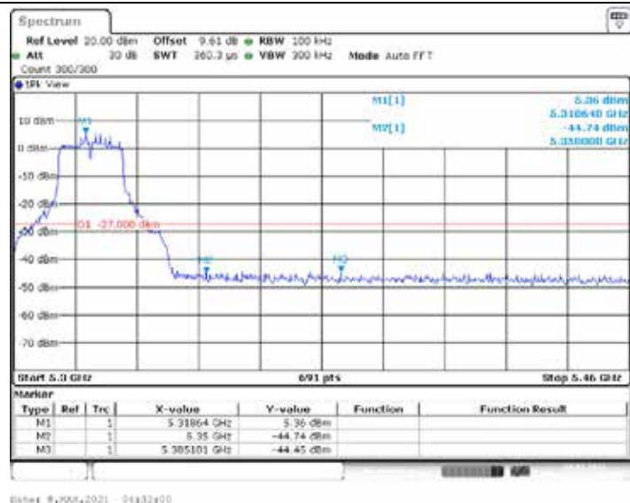
11A_Ant2_High_5320
