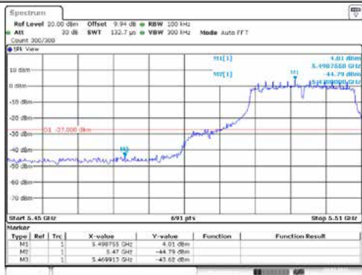
11AC20ISO_Ant2_Low_5500
