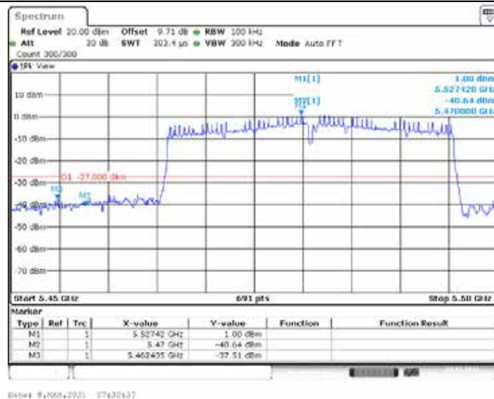
11AC80ISO_Ant1_Low_5530
