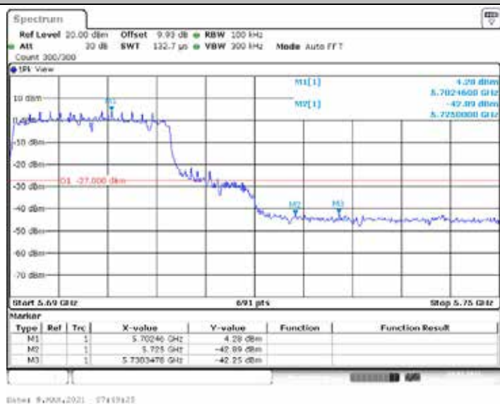
11AX20ISO_Ant1_High_5700
