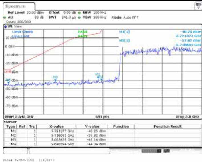
11AX80ISO_Ant1_High_5775
