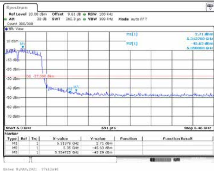
11AC40ISO_Ant1_High_5310
