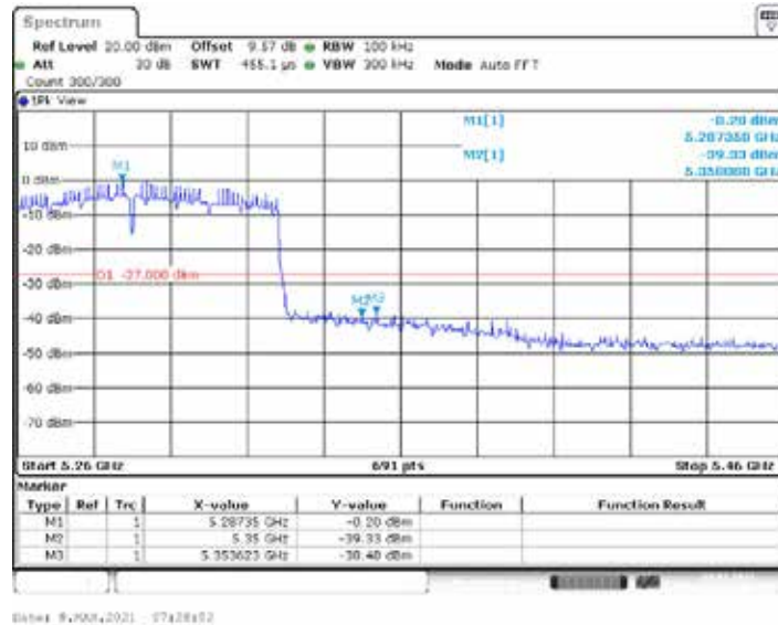
11AC80ISO_Ant2_High_5290
