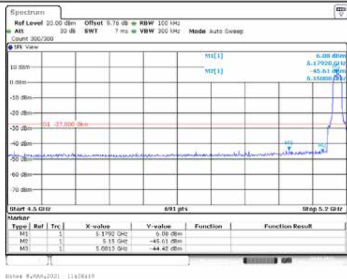
11N20ISO_Ant2_Low_5180
