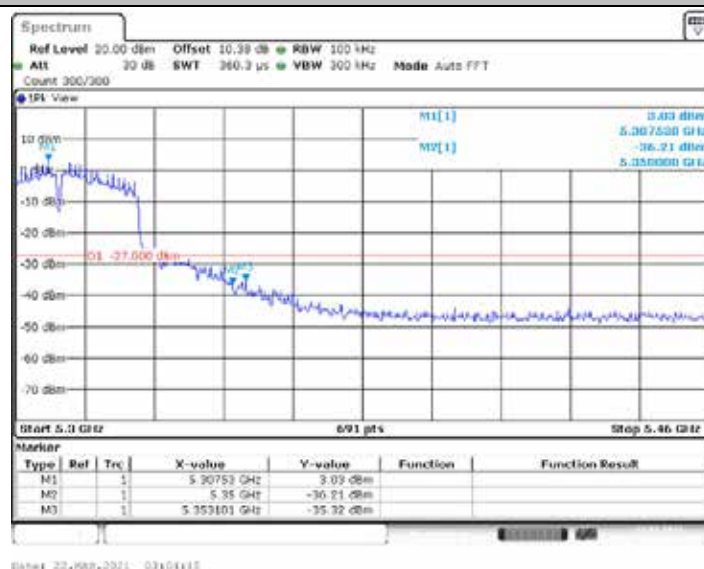
11AC40MIMO_Ant2_High_5310
