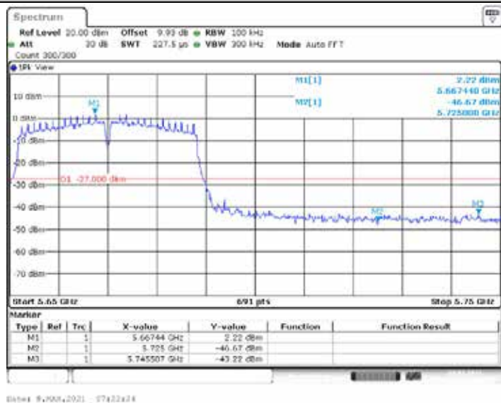
11AC40SISO_Ant2_High_5670
