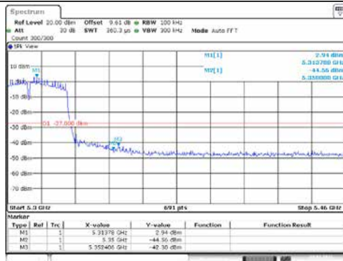
11N40SISO_Ant1_High_5310
