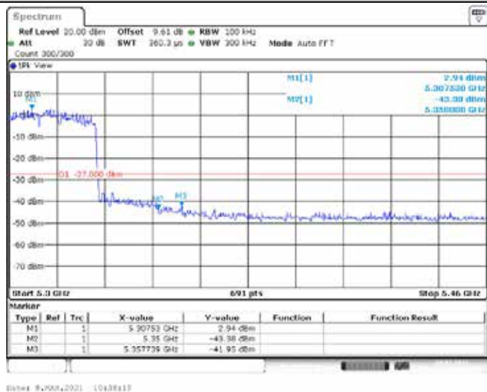
11AX40SISO_Ant2_High_5310
