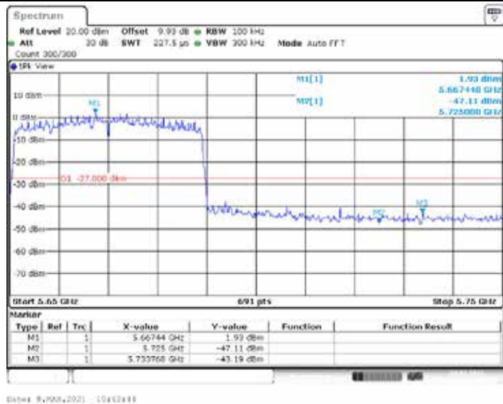
11AX40ISO_Ant2_High_5670
