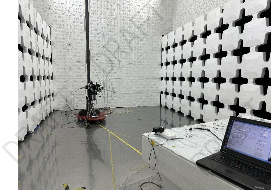
Radiated Emission Above 1G
