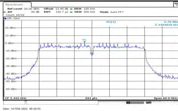
11N40SISO_Ant1_2452_0~Reference
