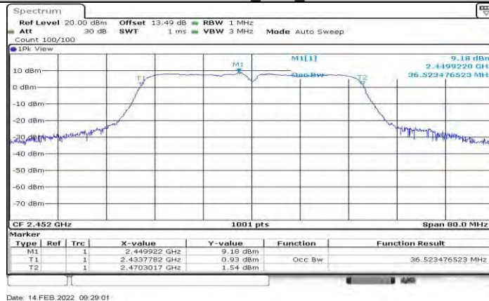
11N40SISO Ant1_2452
