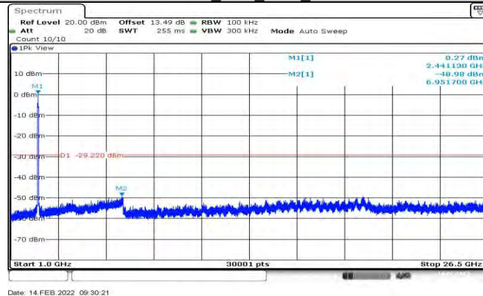
11N40SISO_Ant1_2452_1000~26500
