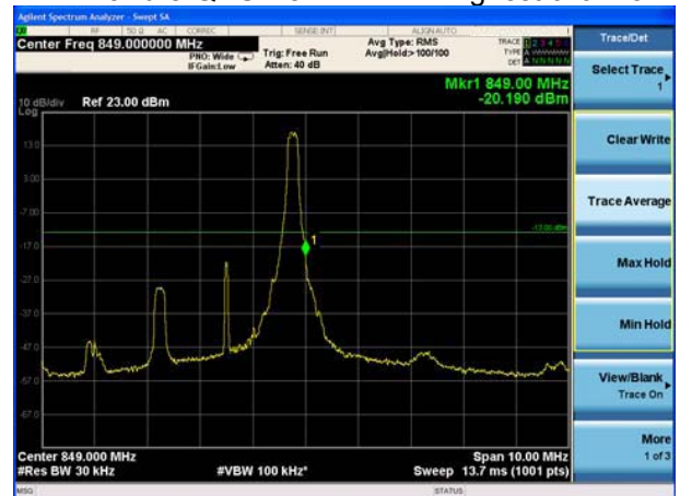
LTE Band 5 QPSK 3MHz 1RB Highest channel
