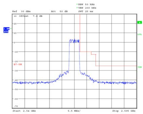
LTE Band 7 16QAM 5MHz 100%RB Highest channel
