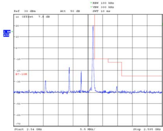
LTE Band 7 16QAM 10MHz 1RB Highest channel:
