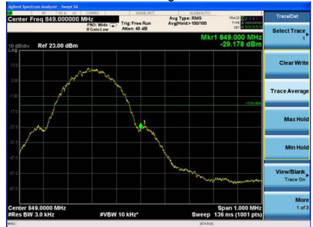
GMSK 850MHz Highest channel
