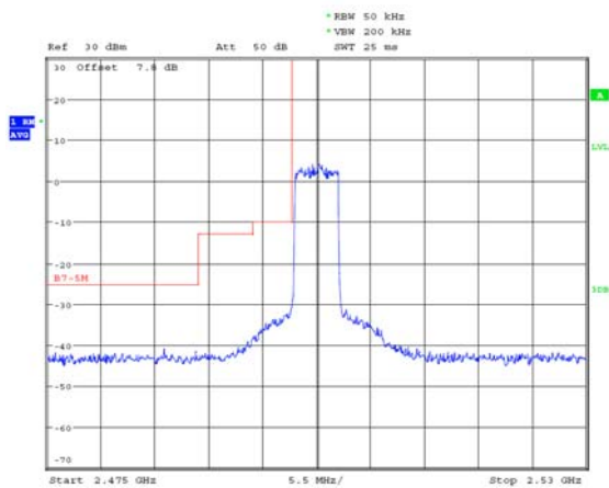
LTE Band 7 16QAM 5MHz 100%RB Lowest channel
