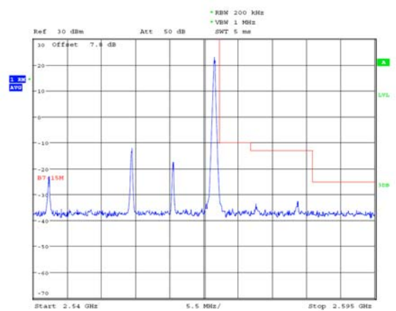
LTE Band 7 QPSK 15MHz 1RB Highest channel:
