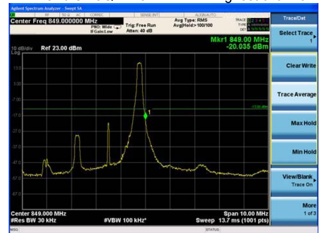
LTE Band 5 16QAM 3MHz 1RB Highest channel:
