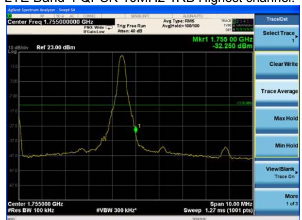
LTE Band 4 QPSK 10MHz 1RB Highest channel:
