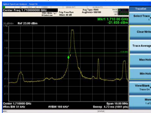
LTE Band 4 QPSK 5MHz 1RB Lowest channel
