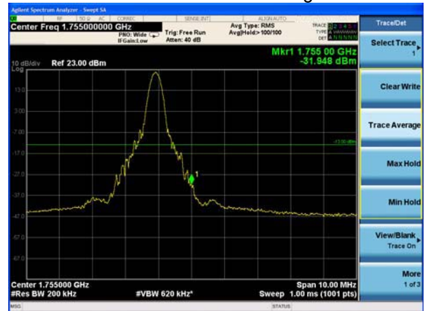
LTE Band 4 16QAM 20MHz 1RB Highest channel:
