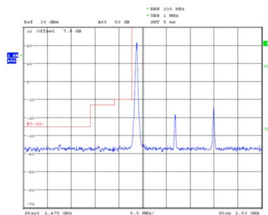
LTE Band 7 16QAM 20MHz 1RB Lowest channel
