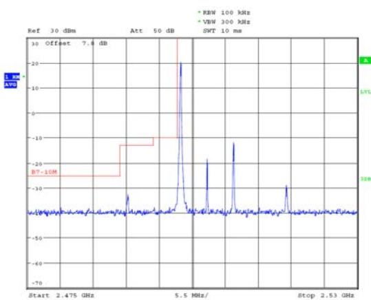
LTE Band 7 16QAM 10MHz 1RB Lowest channel
