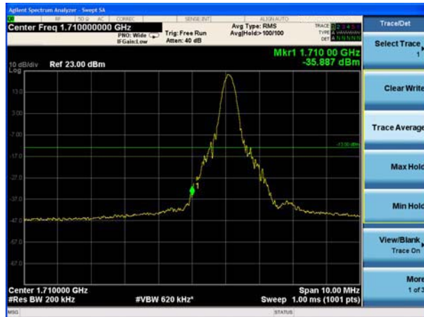
LTE Band 4 16QAM 20MHz 1RB Lowest channel
