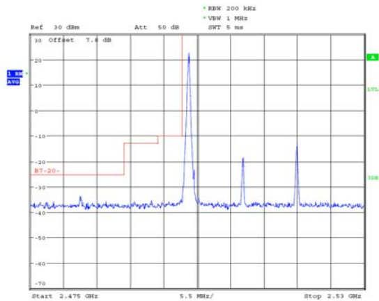
LTE Band 7 QPSK 20MHz 1RB Lowest channel
