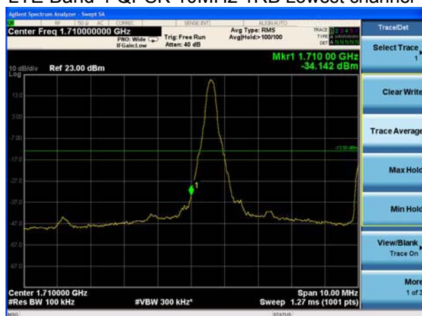
LTE Band 4 QPSK 10MHz 1RB Lowest channel
