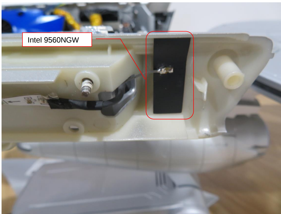
Internal View of EUT-38
