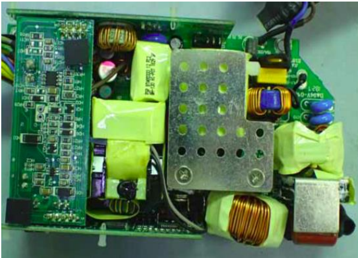
Internal View of EUT-32
