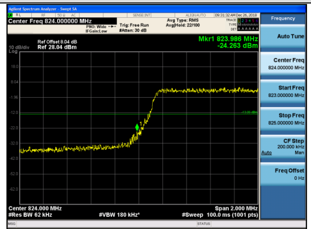
LCH_16QAM_15RB#0
