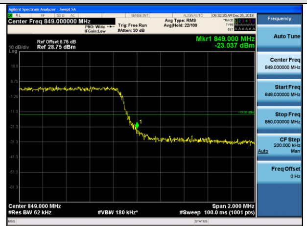
HCH_16QAM_15RB#0
