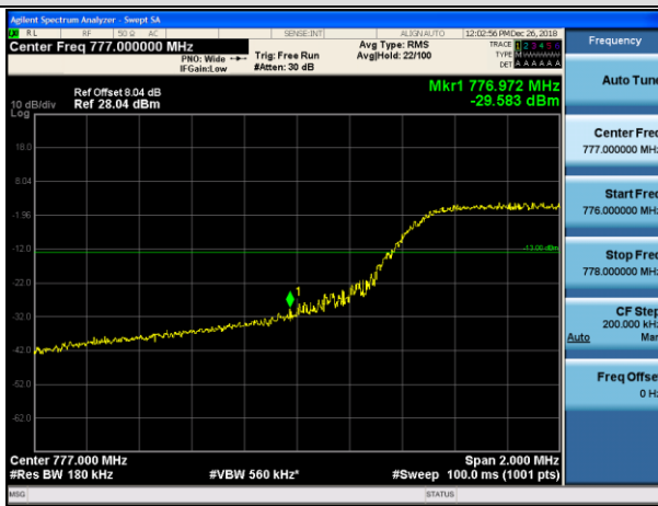
LCH_QPSK_50RB#0
