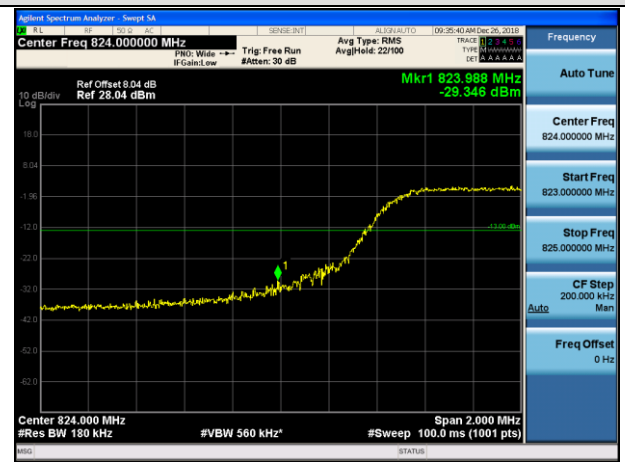
LCH_16QAM_50RB#0
