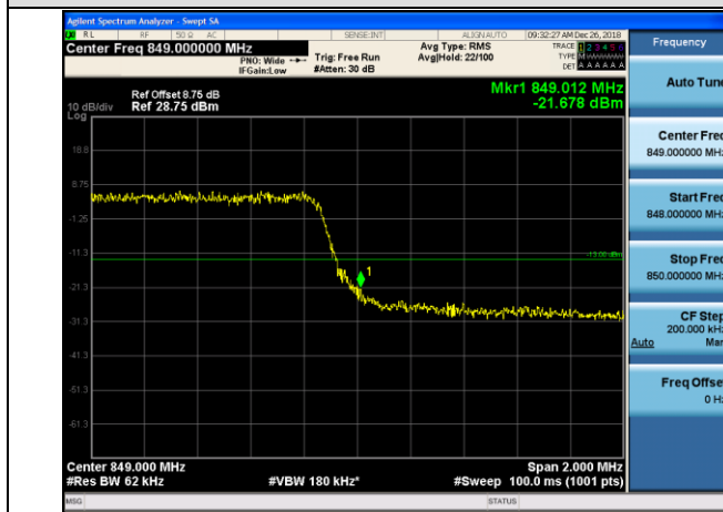
HCH_QPSK_15RB#0
