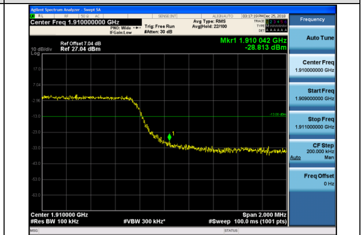
HCH_16QAM_25RB#0
