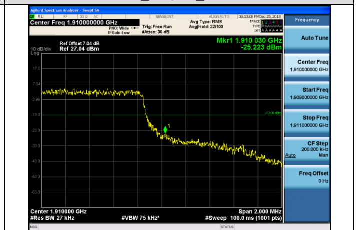
HCH_16QAM_6RB#0
