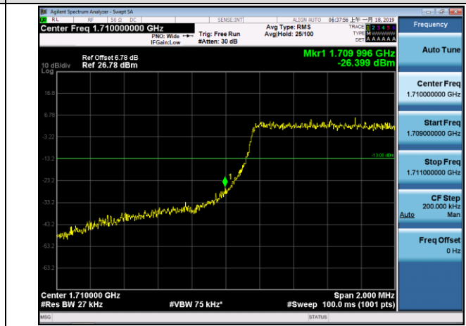
LCH_16QAM_6RB#0
