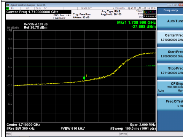
LCH_QPSK_75RB#0
