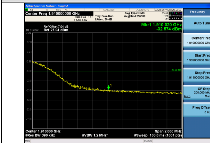
HCH_QPSK_100RB#0
