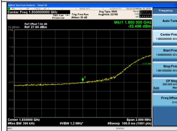
LCH_QPSK_100RB#0
