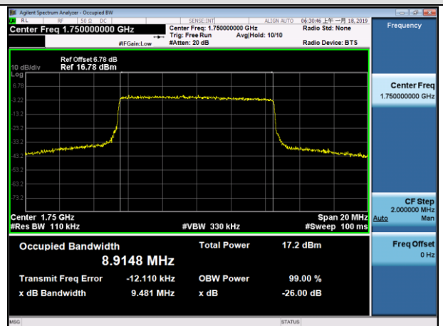
HCH_16QAM_50RB#0
