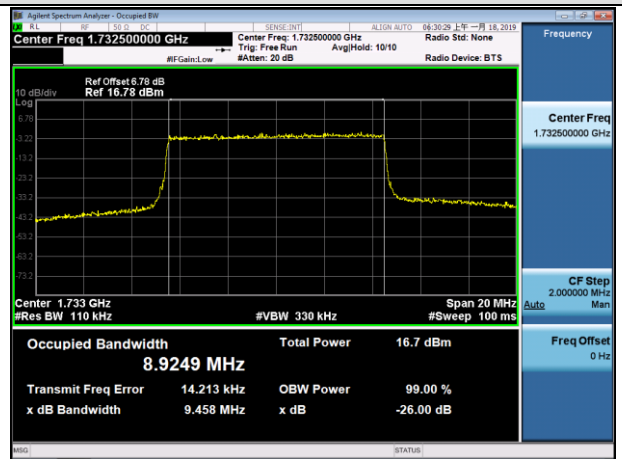
MCH_16QAM_50RB#0
