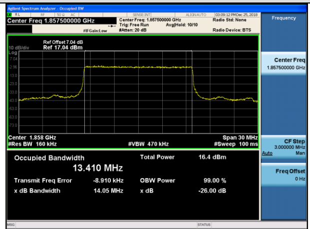
LCH_16QAM_75RB#0
