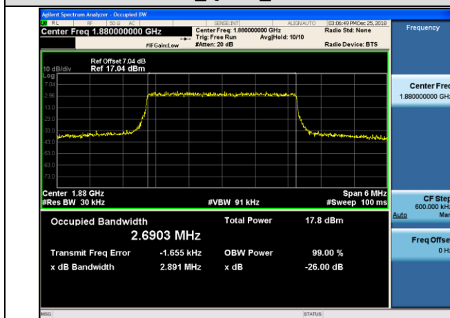
MCH_QPSK_15RB#0
