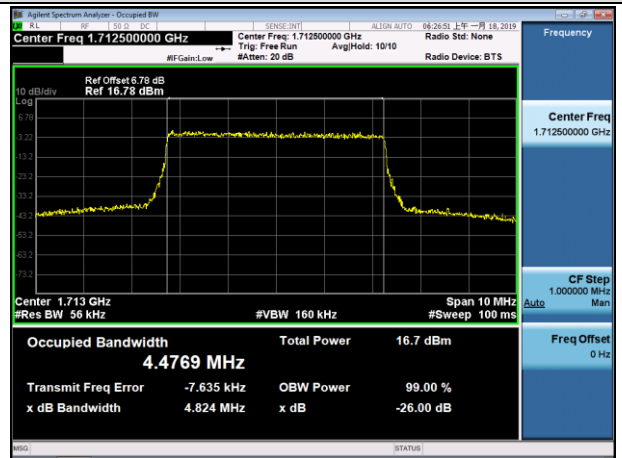
LCH_16QAM_25RB#0
