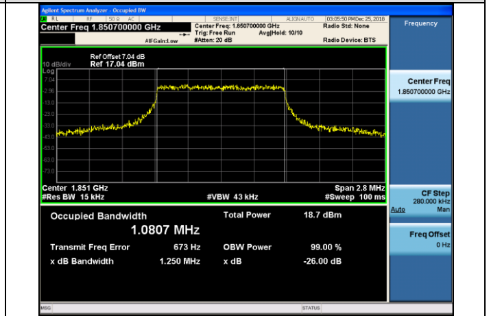
LCH_16QAM_6RB#0
