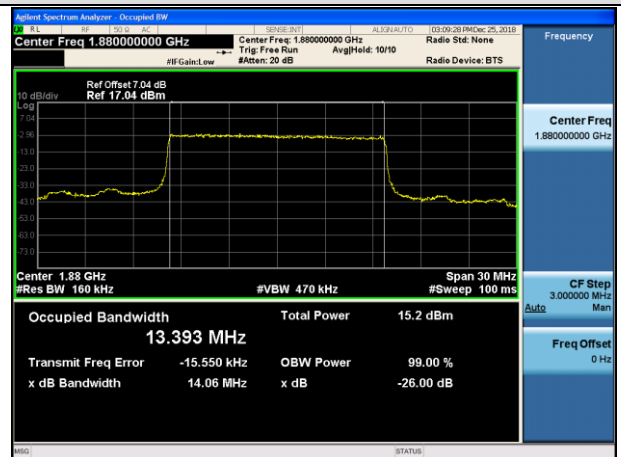
MCH_16QAM_75RB#0
