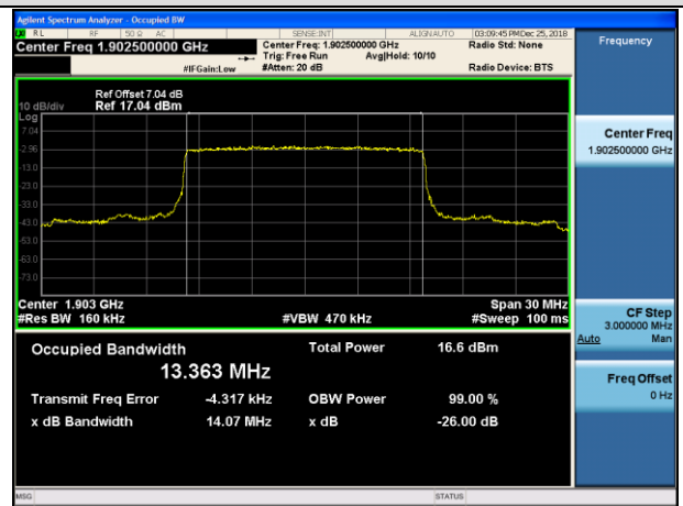
HCH_16QAM_75RB#0
