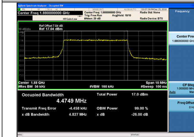
MCH_QPSK_25RB#0
