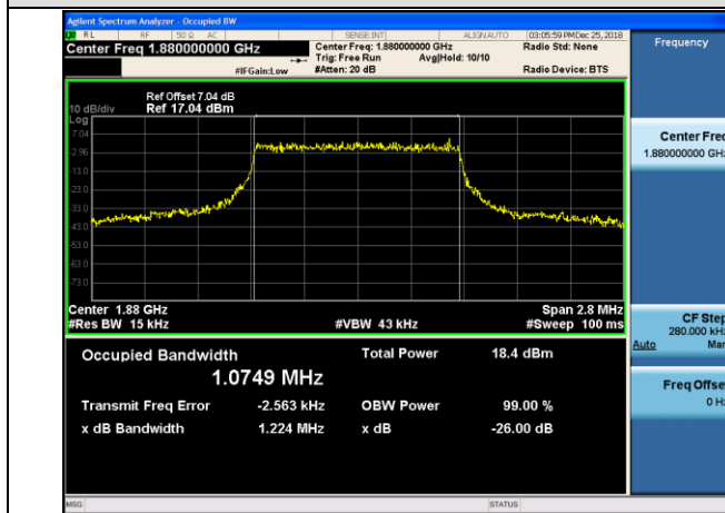
MCH_QPSK_6RB#0
