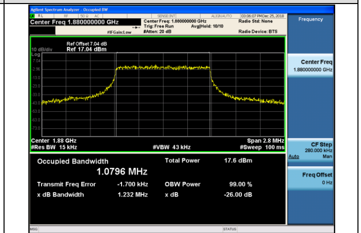
MCH_16QAM_6RB#0
