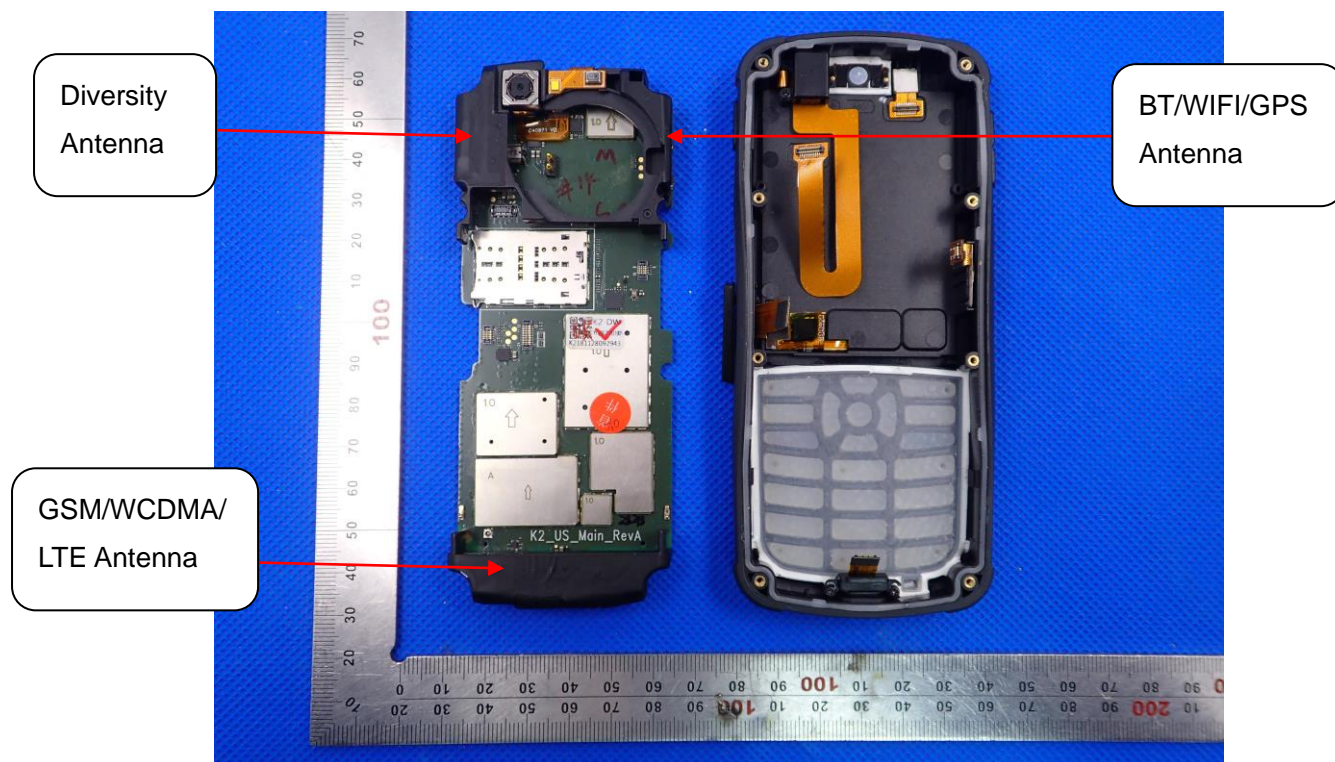
WIFI&BT&GPS ANTENNA
