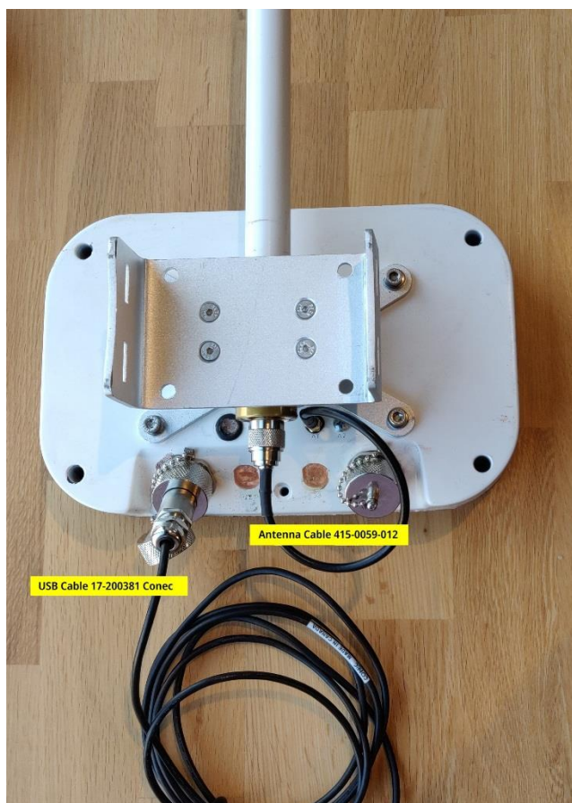
Photograph 7.6.1 Antenna assembly
