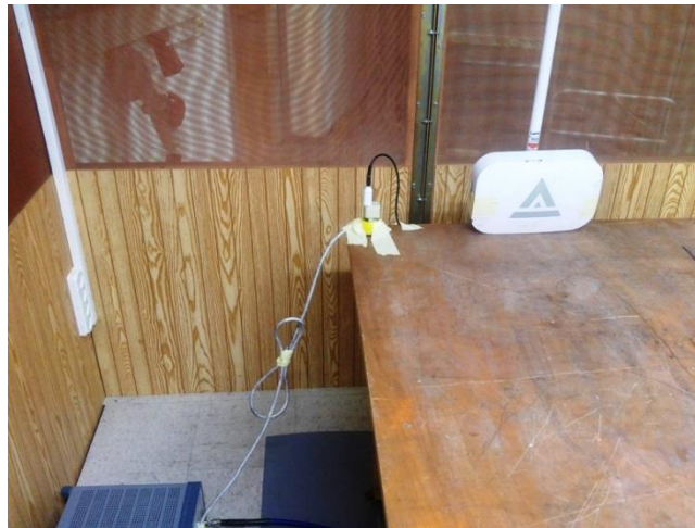
Photograph 8.1.1 Setup for conducted emission measurements
