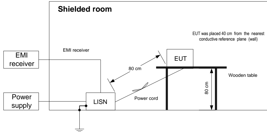
Figure 8.1.1 Setup for conducted emission measurements
