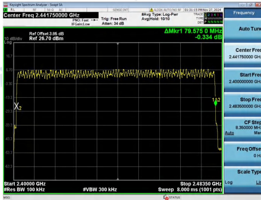
Number_of_Hopping_Channel_(Hopping)_NVNT_ANT1_3-DH5_Hopping
