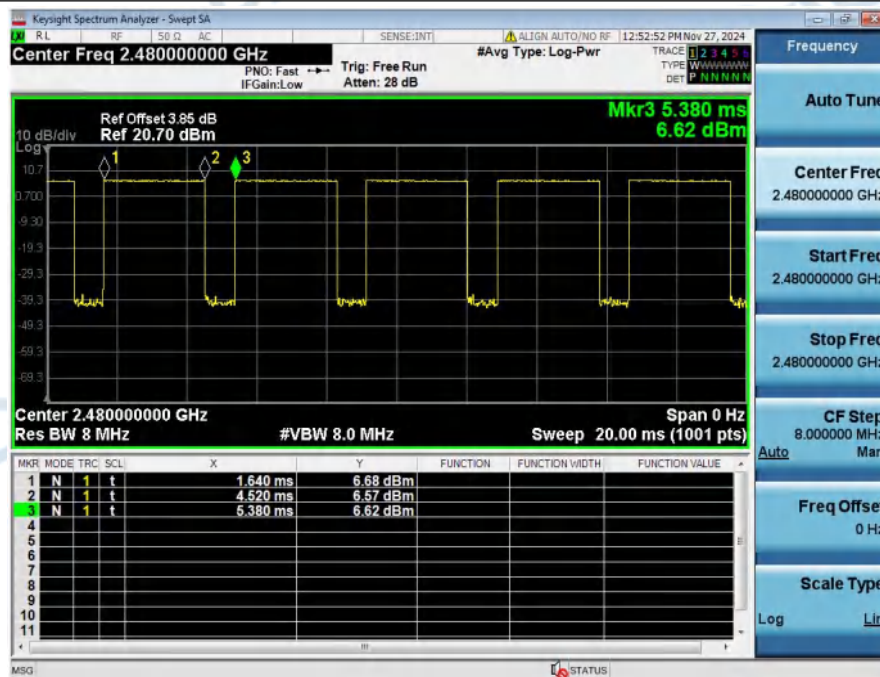
Duty_Cycle_NVNT_ANT1_1-DH5_2480
