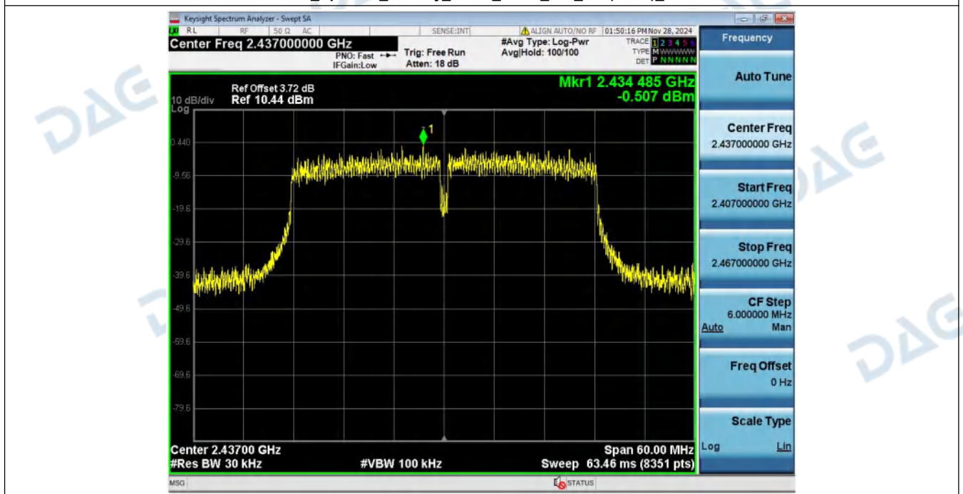
Power_Spectral_Density_NVNT_ANT1_802_11n(HT40)_2437
