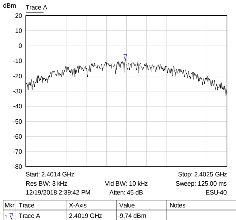
Graph 11: Lowest Channel 3 kHz PSD Plot
