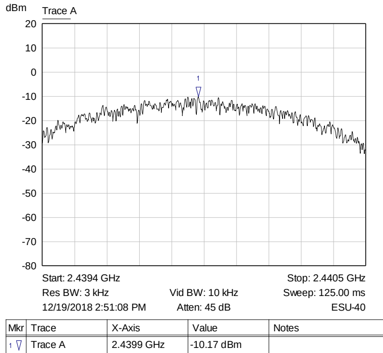
Graph 12: Middle Channel 3 kHz PSD Plot
