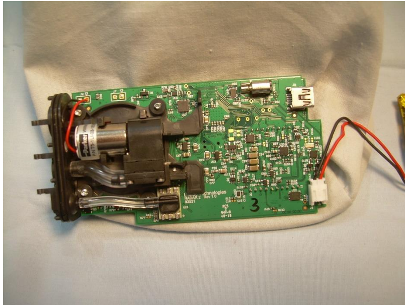
Photograph 19 – Side B of PCB, Battery Holder in Removed
