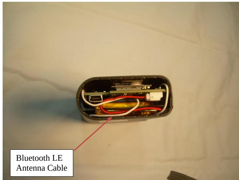
Photograph 15 – Components Inside Housing
