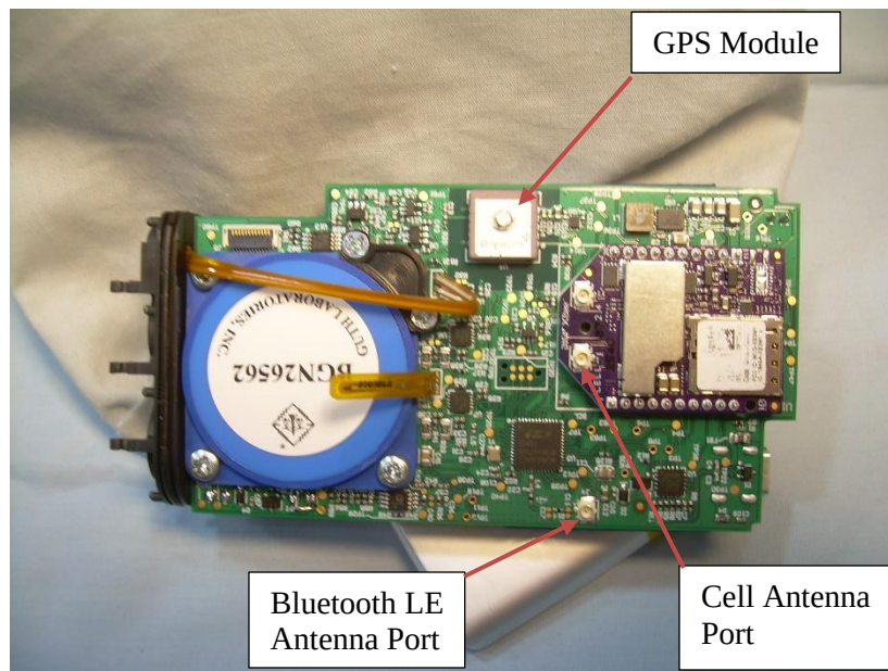
Photograph 16 – Side A of PCB
