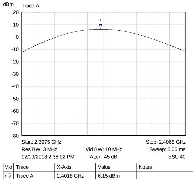
Graph 4: Lowest Channel Output Power Plot
