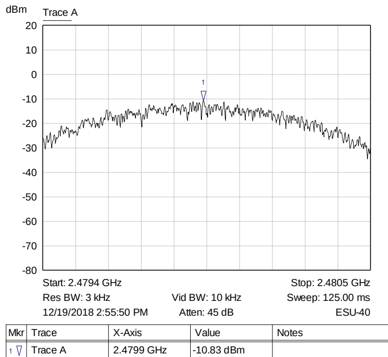
Graph 13: Highest Channel Output 3 kHz PSD Plot
