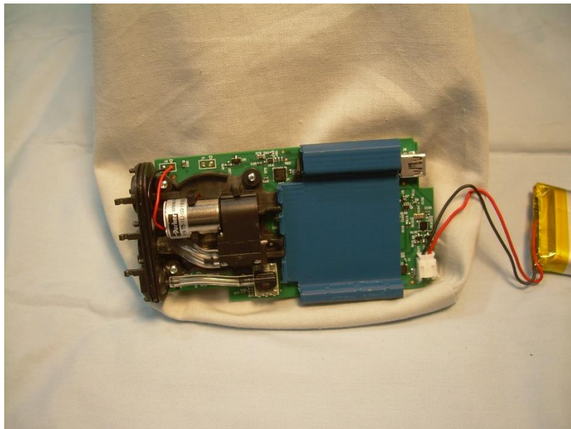
Photograph 18 – Side B of PCB, Battery Holder in Place
