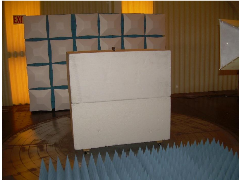
Photograph 5: Front View Radiated Emissions Configuration – Above 1000 MHz – On Edge Battery Powered
