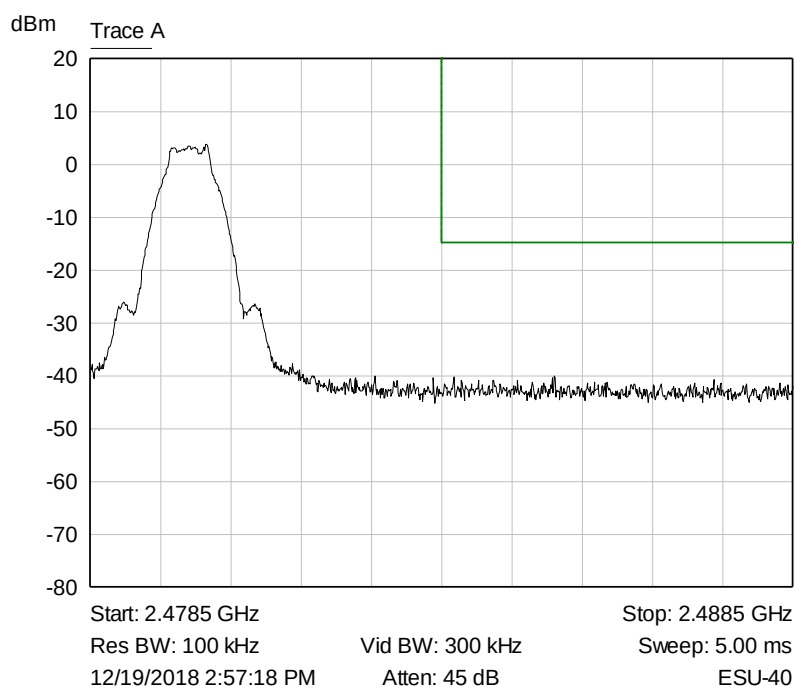
Graph 8: Upper Band Edge Plot
