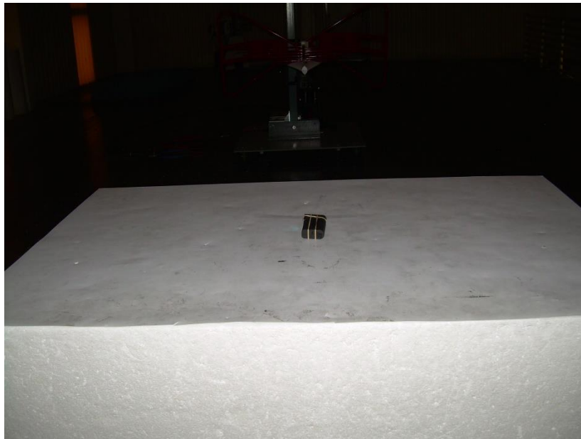
Photograph 2: Back View Radiated Emissions Configuration – 30 to 1000 MHz – Flat Battery Powered
