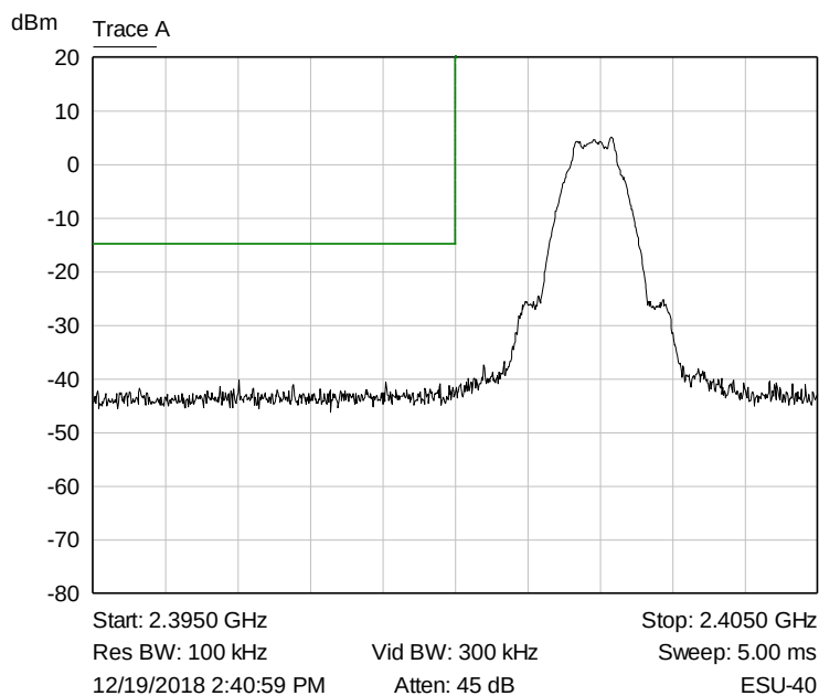
Graph 7: Lower Band Edge Plot
