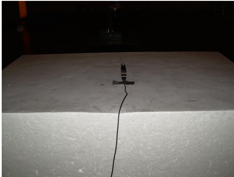
Photograph 4: Back View Radiated Emissions Configuration – 30 to 1000 MHz – On Edge AC Supply Powered
