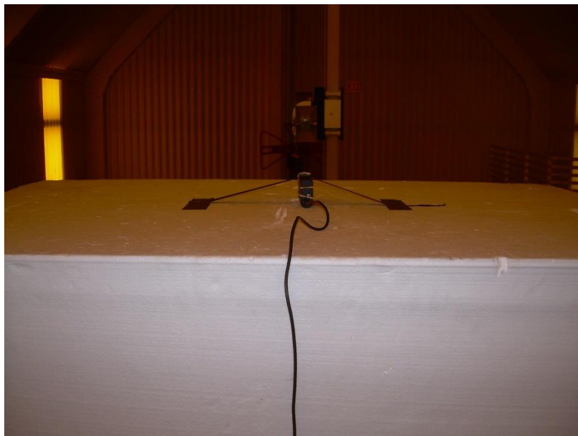
Photograph 6: Back View Radiated Emissions Configuration – Above 1000 MHz – On Edge AC Supply Powered
