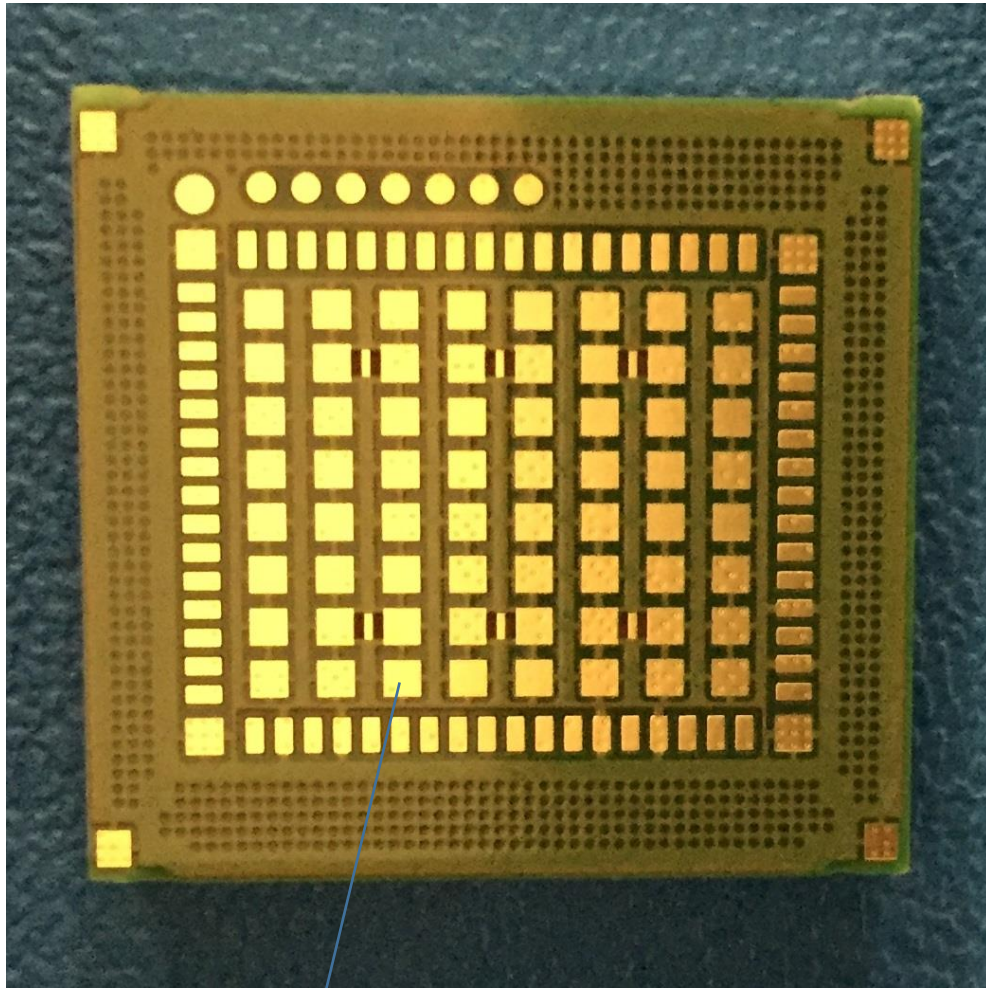
Sierra Wireless HL7618RD Module- contact side
