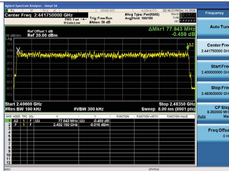
8DPSK Modulation
