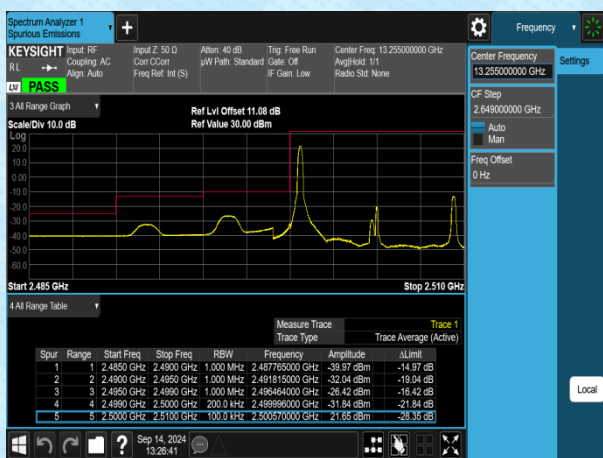
Band7-10MHz-QPSK-20800-1RB#0-PASS
