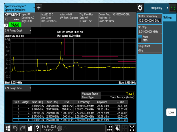
Band7-15MHz-QPSK-21375-1RB#74-PASS
