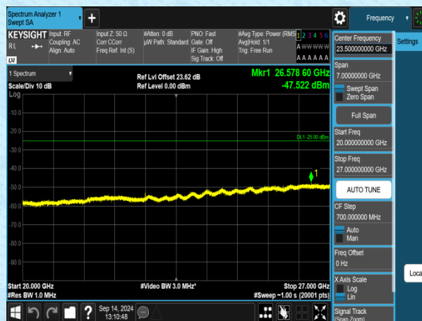
Band7-5MHz-QPSK-21100-1RB#0-20000~27000-PASS
