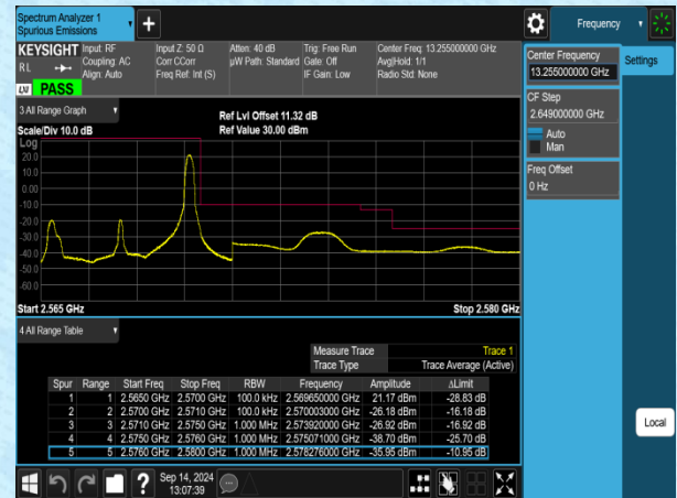
Band7-5MHz-16QAM-21425-1RB#24-PASS
