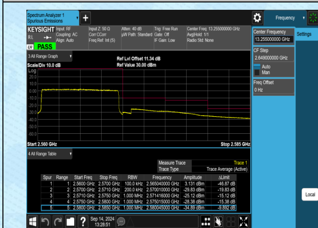
Band7-10MHz-16QAM-21400-50RB#0-PASS
