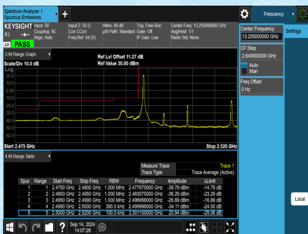
Band7-20MHz-16QAM-20850-1RB#0-PASS
