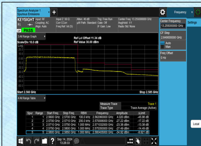
Band7-10MHz-QPSK-21400-50RB#0-PASS
