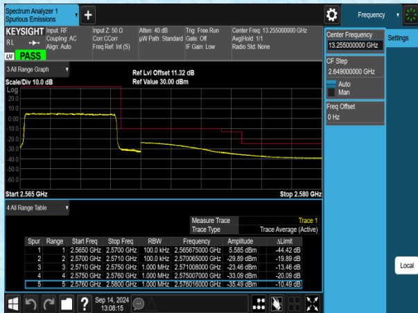
Band7-5MHz-16QAM-21425-25RB#0-PASS
