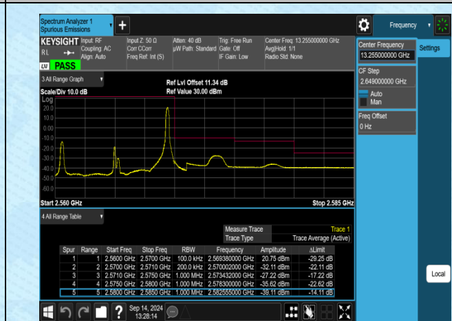
Band7-10MHz-16QAM-21400-1RB#49-PASS
