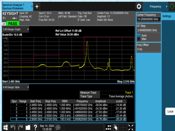
Band7-10MHz-16QAM-20800-1RB#0-PASS
