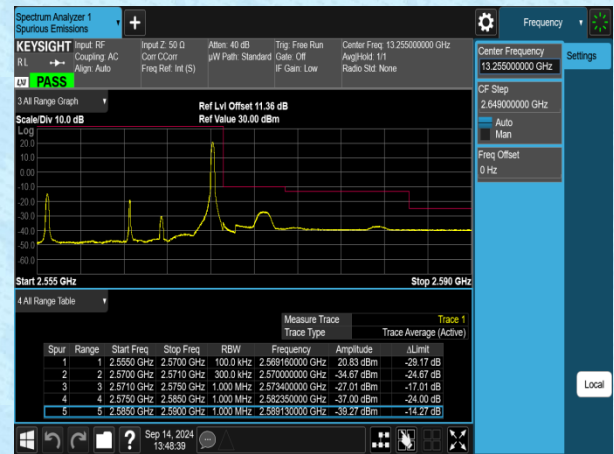
Band7-15MHz-16QAM-21375-1RB#74-PASS
