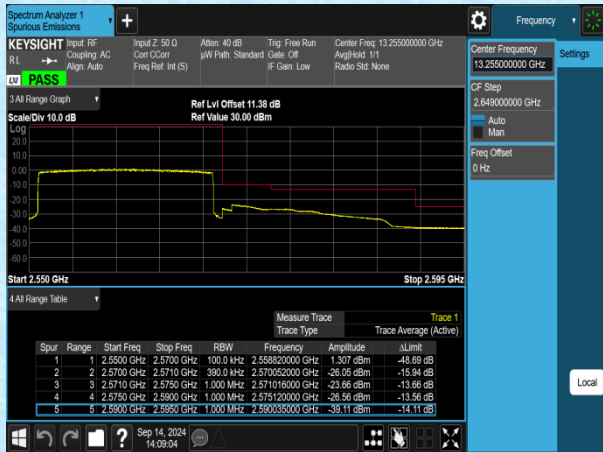
Band7-20MHz-QPSK-21350-100RB#0-PASS
