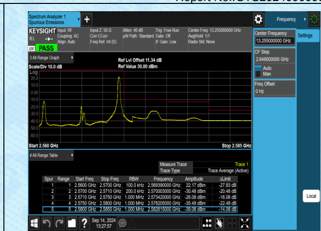
Band7-10MHz-QPSK-21400-1RB#49-PASS
