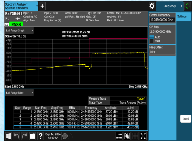
Band7-15MHz-16QAM-20825-75RB#0-PASS
