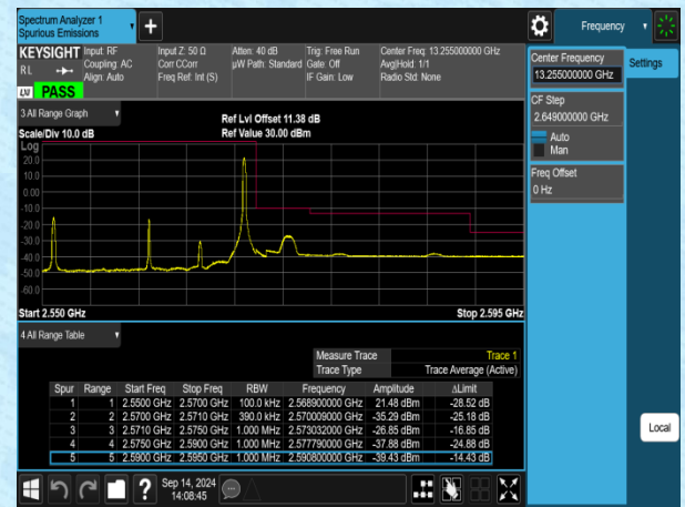
Band7-20MHz-16QAM-21350-1RB#99-PASS
