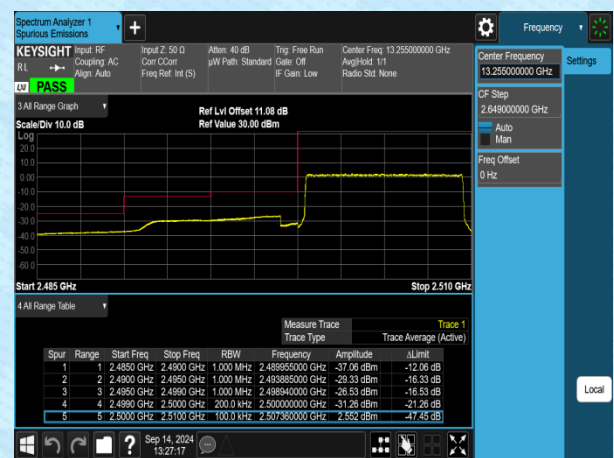
Band7-10MHz-QPSK-20800-50RB#0-PASS
