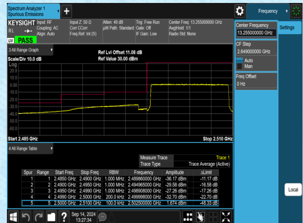
Band7-10MHz-16QAM-20800-50RB#0-PASS
