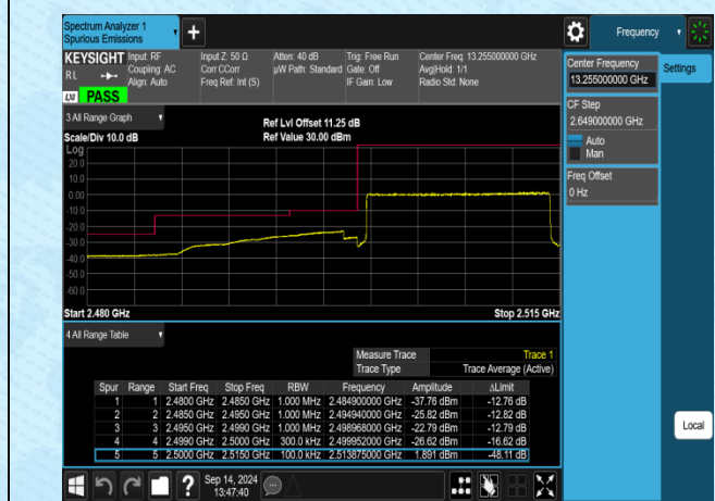
Band7-15MHz-QPSK-20825-75RB#0-PASS
