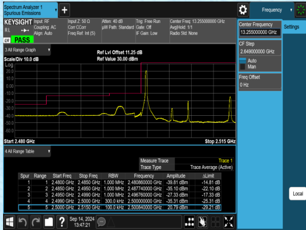
Band7-15MHz-16QAM-20825-1RB#0-PASS
