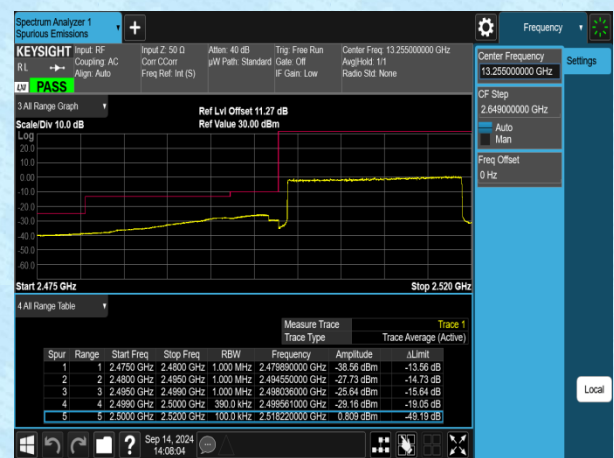
Band7-20MHz-16QAM-20850-100RB#0-PASS
