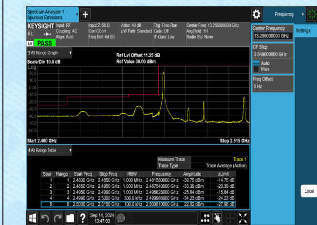
Band7-15MHz-QPSK-20825-1RB#0-PASS
