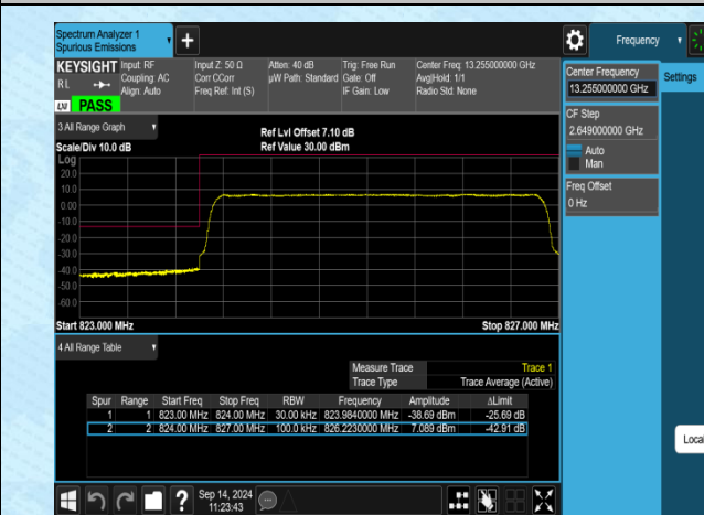
Band5-3MHz-QPSK-20415-15RB#0-PASS
