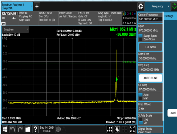
Band5-1.4MHz-QPSK-20643-1RB#0-30~1000-PASS
