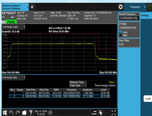
Band5-5MHz-QPSK-20625-25RB#0-PASS
