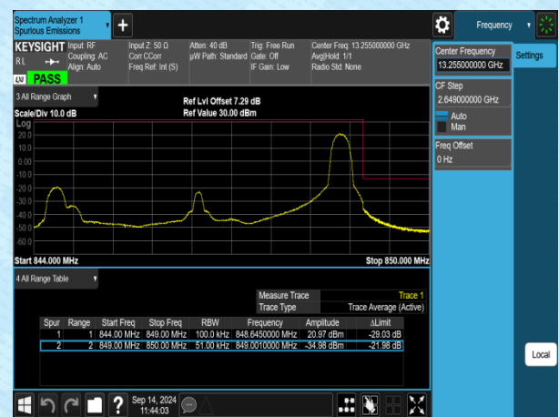
Band5-5MHz-QPSK-20625-1RB#24-PASS
