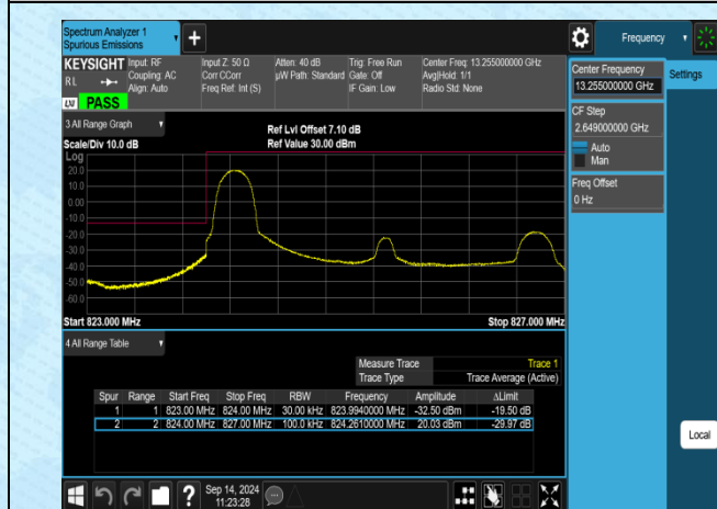
Band5-3MHz-16QAM-20415-1RB#0-PASS
