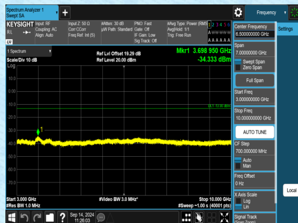
Band5-3MHz-QPSK-20415-1RB#0-3000~10000-PASS
