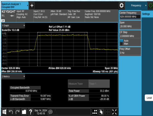
Band5-10MHz-QPSK-20450-50RB#0-PASS
