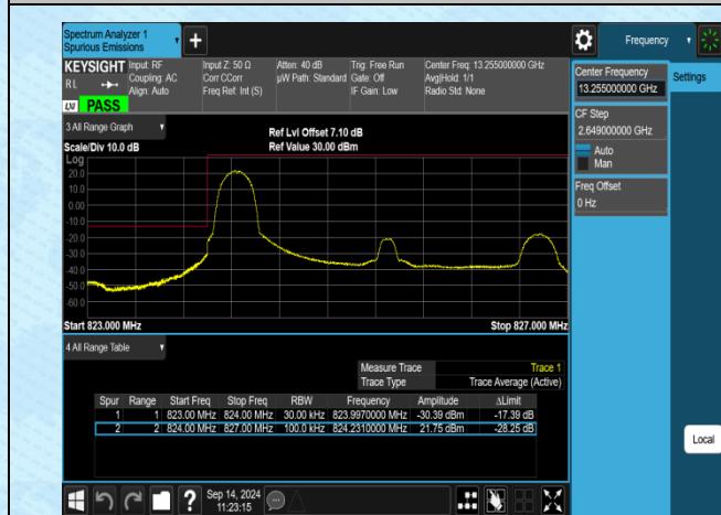
Band5-3MHz-QPSK-20415-1RB#0-PASS
