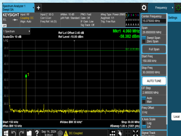
Band5-1.4MHz-QPSK-20525-1RB#0-0.15~30-PASS
