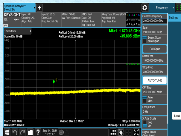
Band5-3MHz-QPSK-20525-1RB#0-1000~3000-PASS
