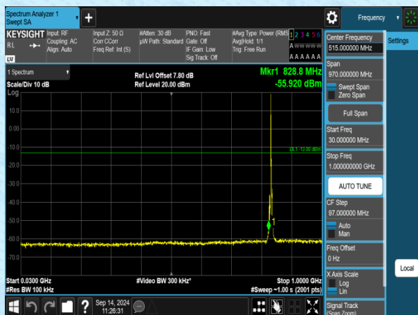
Band5-3MHz-QPSK-20525-1RB#0-30~1000-PASS
