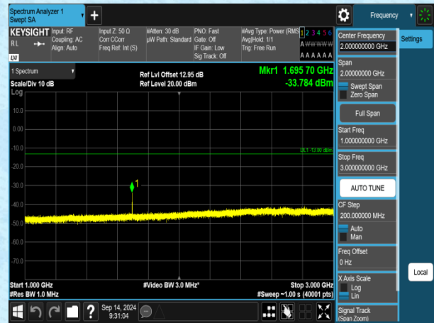
Band5-1.4MHz-QPSK-20643-1RB#0-1000~3000-PASS
