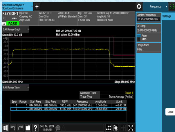
Band5-5MHz-16QAM-20625-25RB#0-PASS
