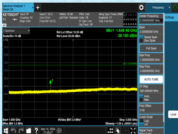
Band5-3MHz-QPSK-20415-1RB#0-1000~3000-PASS
