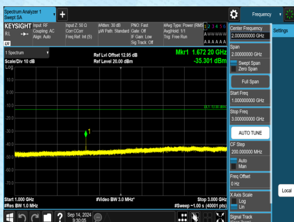
Band5-1.4MHz-QPSK-20525-1RB#0-1000~3000-PASS
