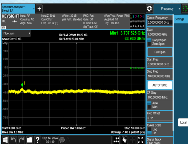
Band5-1.4MHz-QPSK-20643-1RB#0-3000~10000-PASS
