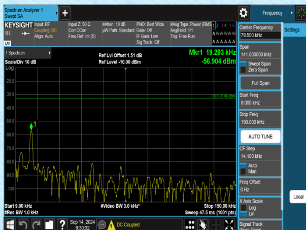
Band5-1.4MHz-QPSK-20643-1RB#0-0.009~0.15-PASS
