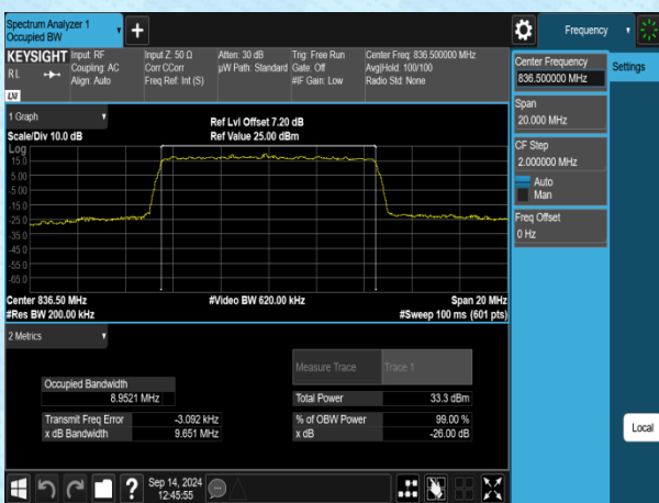
Band5-10MHz-QPSK-20525-50RB#0-PASS
