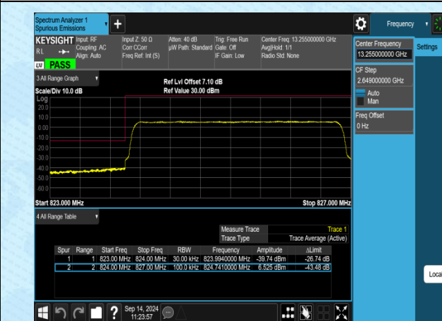
Band5-3MHz-16QAM-20415-15RB#0-PASS
