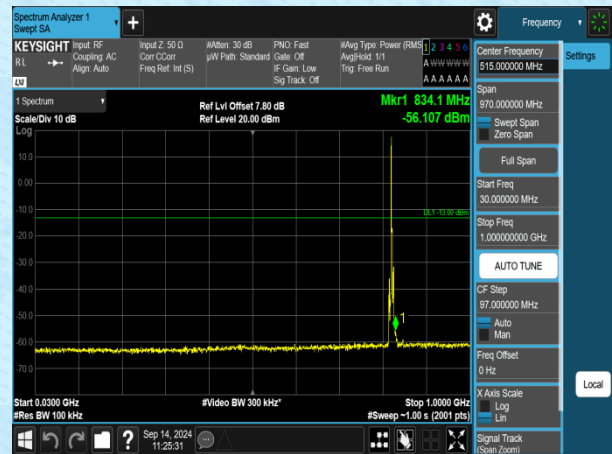
Band5-3MHz-QPSK-20415-1RB#0-30~1000-PASS
