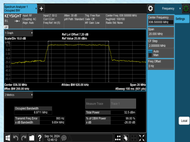
Band5-10MHz-16QAM-20525-50RB#0-PASS
