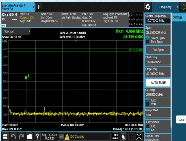
Band5-3MHz-QPSK-20415-1RB#0-0.15~30-PASS
