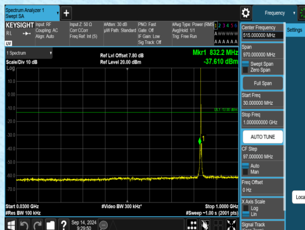
Band5-1.4MHz-QPSK-20525-1RB#0-30~1000-PASS
