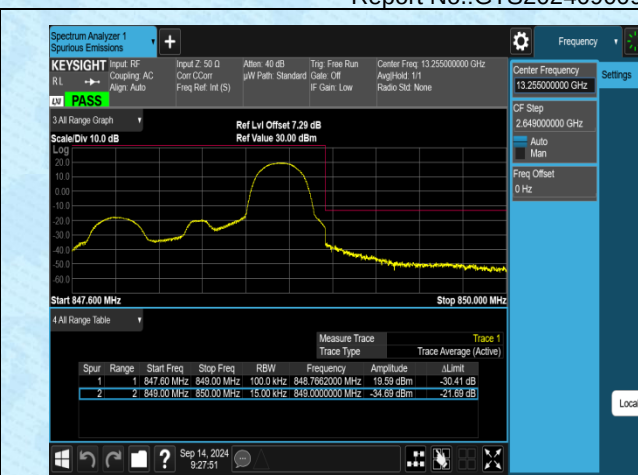
Band5-1.4MHz-16QAM-20643-1RB#5-PASS
