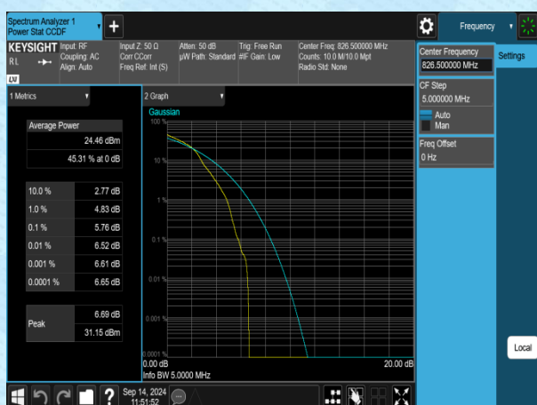
Band5-5MHz-16QAM-20425-1RB#0-PASS
