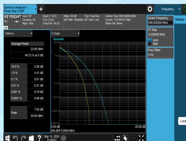
Band5-5MHz-QPSK-20625-25RB#0-PASS
