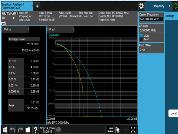
Band5-3MHz-16QAM-20635-1RB#0-PASS
