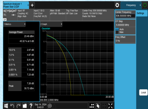
Band5-1.4MHz-16QAM-20525-6RB#0-PASS
