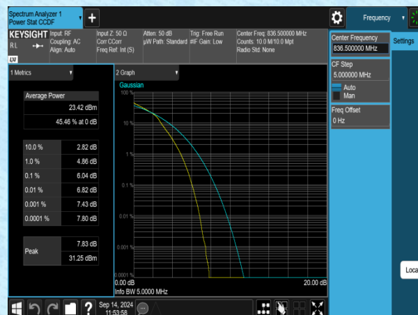
Band5-5MHz-16QAM-20525-25RB#0-PASS
