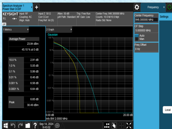
Band5-1.4MHz-16QAM-20643-1RB#0-PASS
