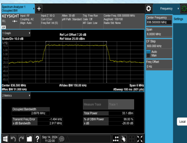
Band5-3MHz-QPSK-20525-15RB#0-PASS
