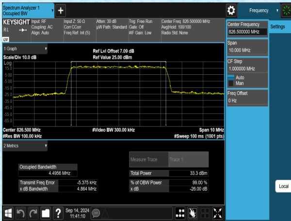
Band5-5MHz-QPSK-20425-25RB#0-PASS
