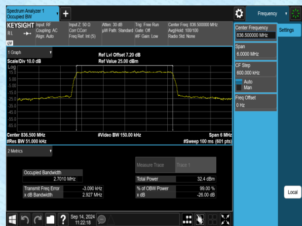
Band5-3MHz-16QAM-20525-15RB#0-PASS
