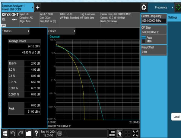
Band5-10MHz-16QAM-20450-1RB#0-PASS
