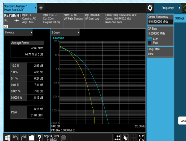
Band5-5MHz-16QAM-20625-25RB#0-PASS
