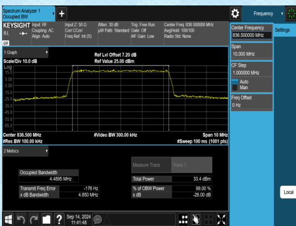
Band5-5MHz-QPSK-20525-25RB#0-PASS
