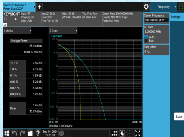
Band5-3MHz-QPSK-20525-1RB#0-PASS
