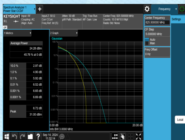
Band5-3MHz-16QAM-20415-1RB#0-PASS
