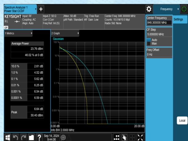
Band5-1.4MHz-QPSK-20643-6RB#0-PASS
