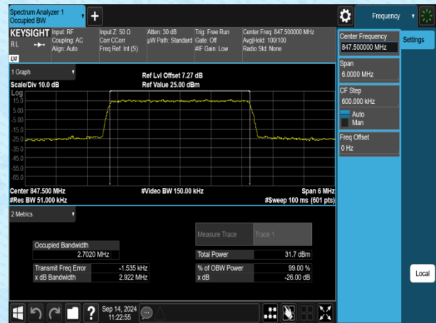
Band5-3MHz-16QAM-20635-15RB#0-PASS
