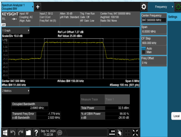
Band5-3MHz-QPSK-20635-15RB#0-PASS
