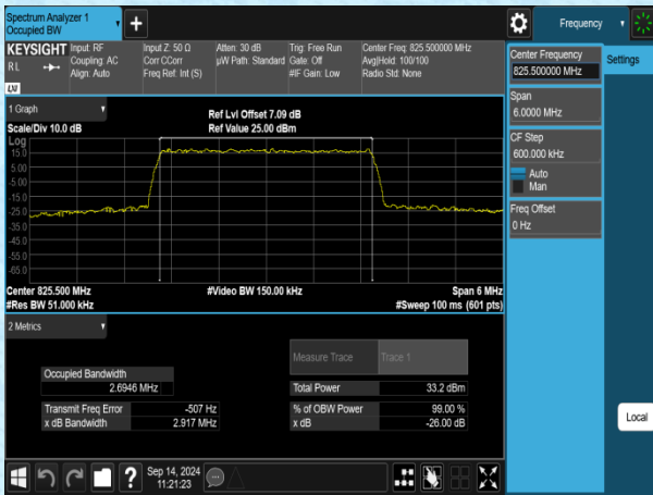
Band5-3MHz-QPSK-20415-15RB#0-PASS
