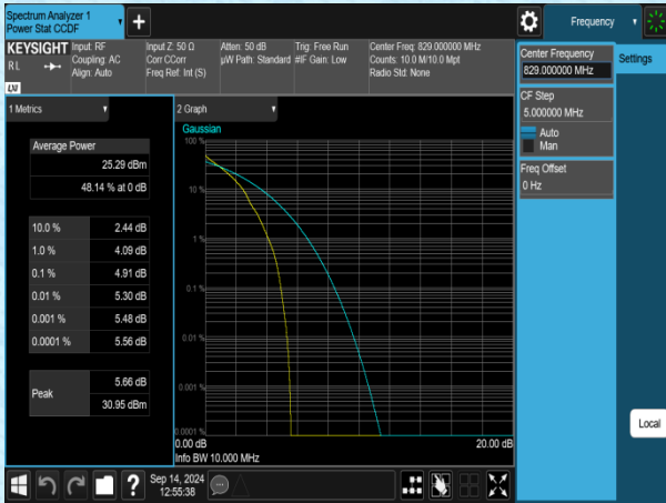
Band5-10MHz-QPSK-20450-1RB#0-PASS
