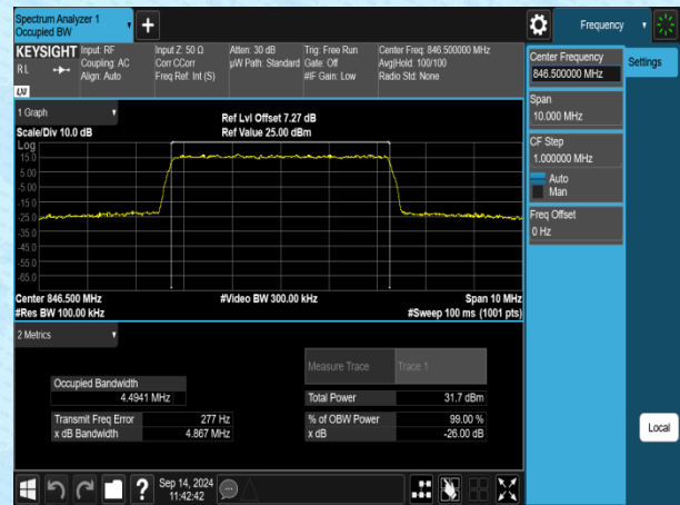
Band5-5MHz-16QAM-20625-25RB#0-PASS
