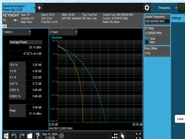
Band5-5MHz-QPSK-20525-1RB#0-PASS
