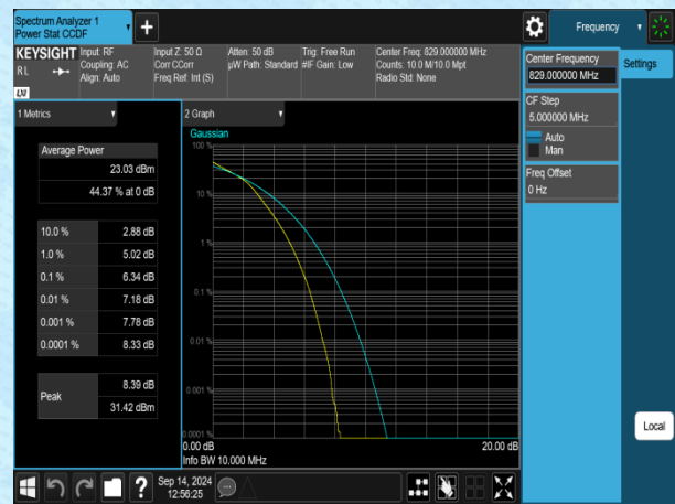
Band5-10MHz-16QAM-20450-50RB#0-PASS
