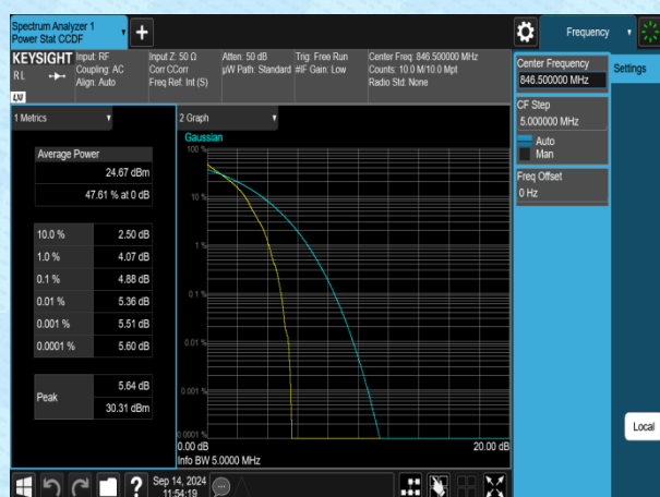
Band5-5MHz-QPSK-20625-1RB#0-PASS
