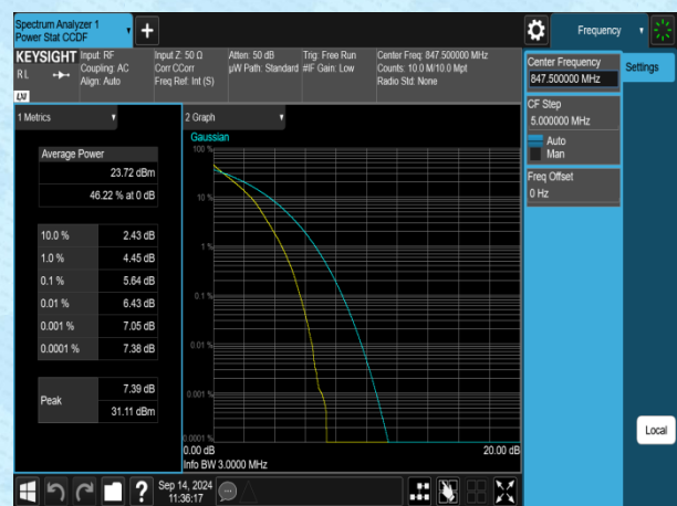
Band5-3MHz-QPSK-20635-15RB#0-PASS
