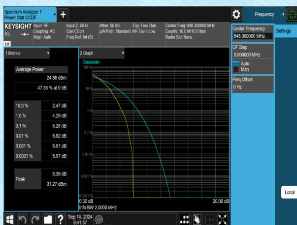
Band5-1.4MHz-QPSK-20643-1RB#0-PASS
