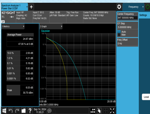
Band5-3MHz-QPSK-20635-1RB#0-PASS
