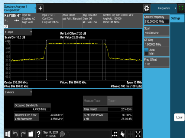
Band5-5MHz-16QAM-20525-25RB#0-PASS
