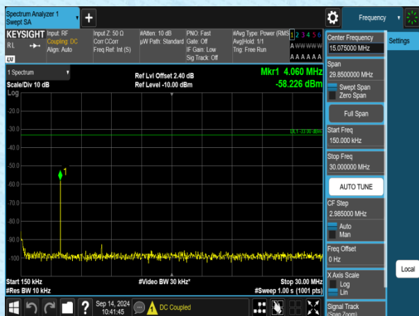
Band4-3MHz-QPSK-19965-1RB#0-0.15~30-PASS
