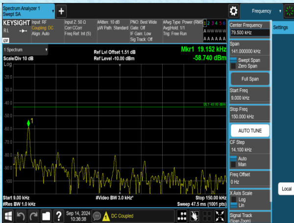
Band4-1.4MHz-QPSK-20393-1RB#0-0.009~0.15-PASS
