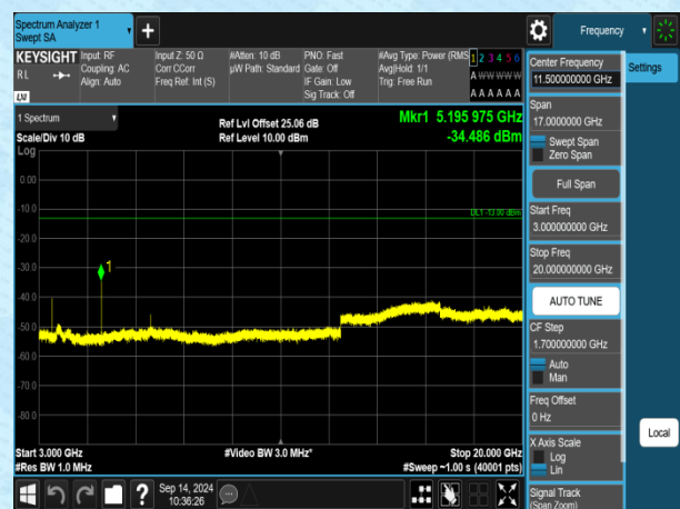
Band4-1.4MHz-QPSK-20175-1RB#0-3000~20000-PASS
