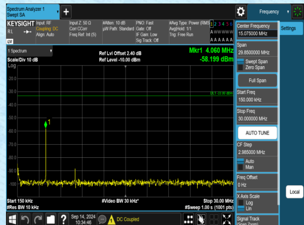
Band4-1.4MHz-QPSK-19957-1RB#0-0.15~30-PASS
