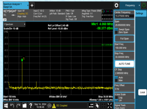
Band4-1.4MHz-QPSK-20393-1RB#0-0.15~30-PASS
