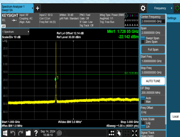
Band4-1.4MHz-QPSK-20175-1RB#0-1000~3000-PASS
