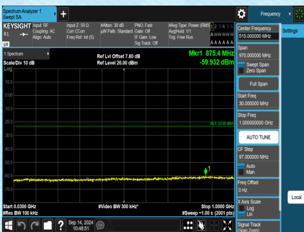
Band4-5MHz-QPSK-19975-1RB#0-30~1000-PASS
