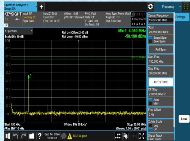
Band4-5MHz-QPSK-19975-1RB#0-0.15~30-PASS
