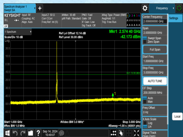
Band4-5MHz-QPSK-19975-1RB#0-1000~3000-PASS
