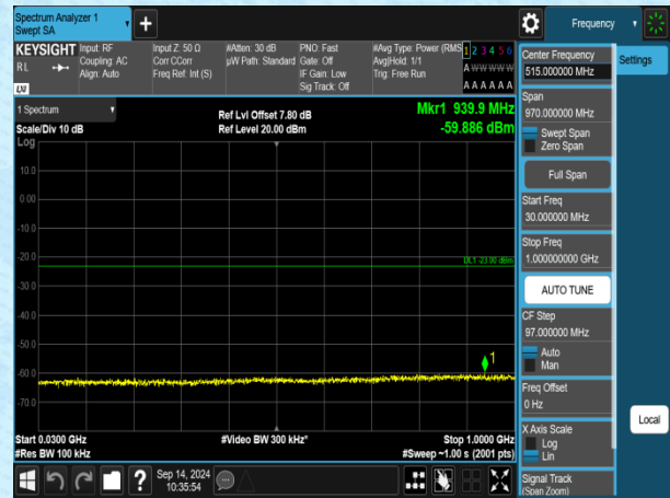
Band4-1.4MHz-QPSK-20175-1RB#0-30~1000-PASS
