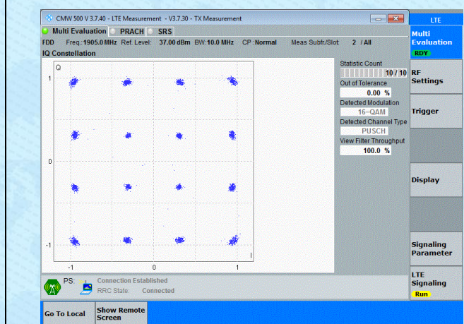
Band2-10MHz-16QAM-19150-50RB#0-PASS
