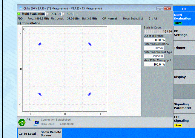
Band2-3MHz-QPSK-19185-15RB#0-PASS
