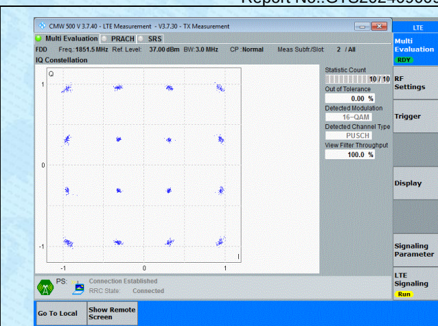
Band2-3MHz-16QAM-18615-15RB#0-PASS
