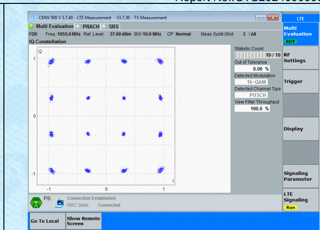
Band2-10MHz-16QAM-18650-50RB#0-PASS
