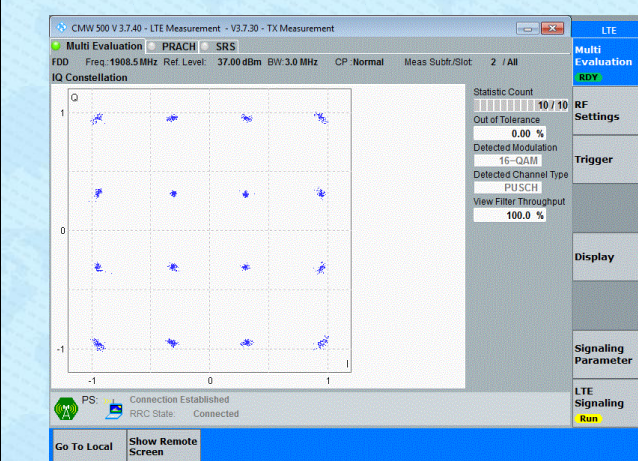
Band2-3MHz-16QAM-19185-15RB#0-PASS
