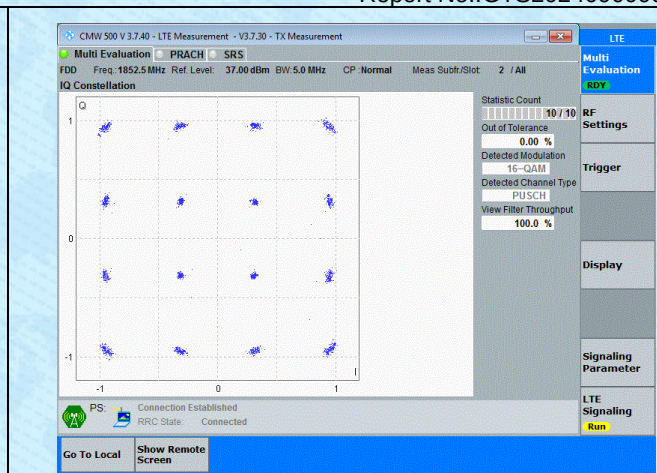
Band2-5MHz-16QAM-18625-25RB#0-PASS
