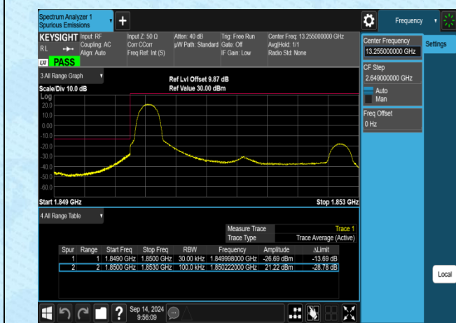
Band2-3MHz-16QAM-18615-1RB#0-PASS
