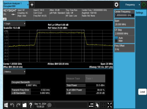
Band2-10MHz-16QAM-18650-50RB#0-PASS
