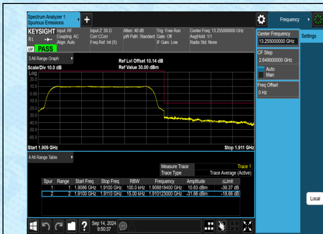
Band2-1.4MHz-16QAM-19193-6RB#0-PASS
