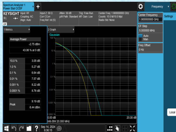
Band2-20MHz-16QAM-19100-100RB#0-PASS
