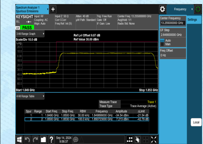
Band2-3MHz-16QAM-18615-15RB#0-PASS
