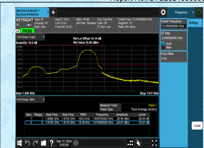
Band2-1.4MHz-16QAM-19193-1RB#5-PASS
