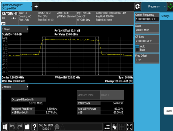
Band2-10MHz-QPSK-19150-50RB#0-PASS
