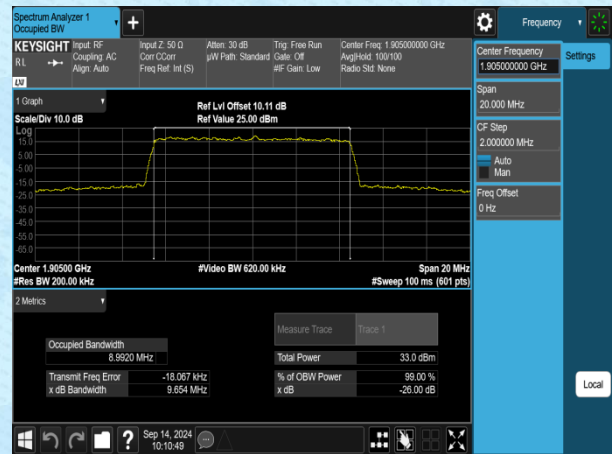
Band2-10MHz-16QAM-19150-50RB#0-PASS
