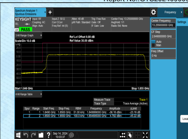
Band2-5MHz-16QAM-18625-25RB#0-PASS
