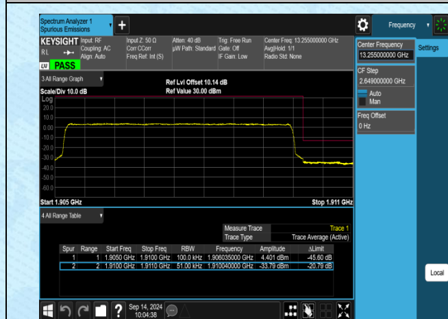
Band2-5MHz-16QAM-19175-25RB#0-PASS
