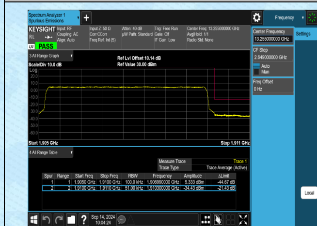
Band2-5MHz-QPSK-19175-25RB#0-PASS
