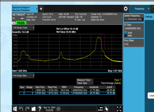
Band2-5MHz-QPSK-19175-1RB#24-PASS
