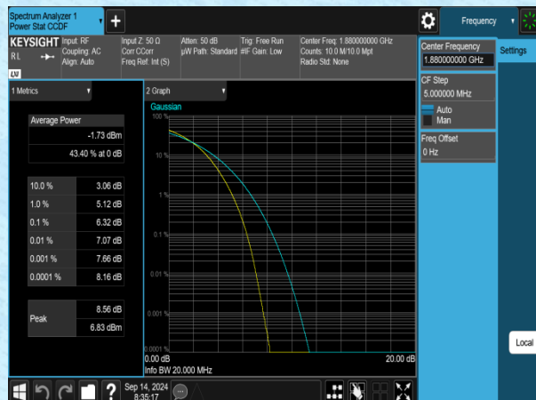
Band2-20MHz-16QAM-18900-100RB#0-PASS
