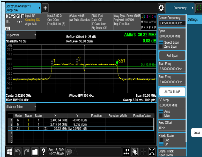
11N40MIMO-Ant1-2422-PASS
