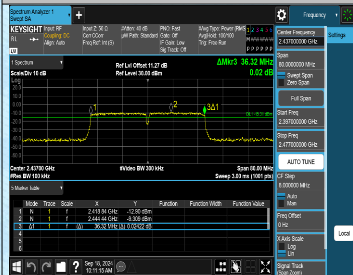
11N40MIMO-Ant1-2437-PASS
