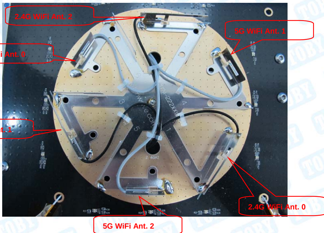
Photo 25 Appearance of WiFi Antenna
