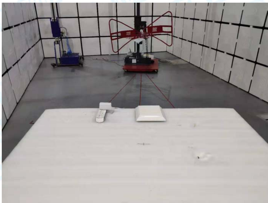
Photo of Setup for Radiated Emission (Below 1 GHz) (Adapter 1#)
