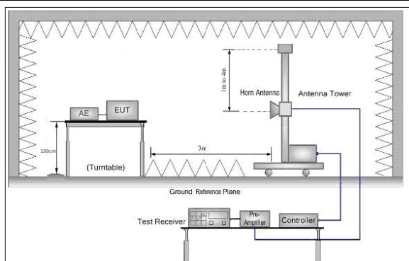
Figure 3. Above 1 GHz
