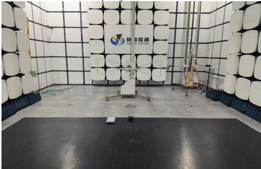
Radiated Spurious Emissions Test Frequency From Below 30MHz
