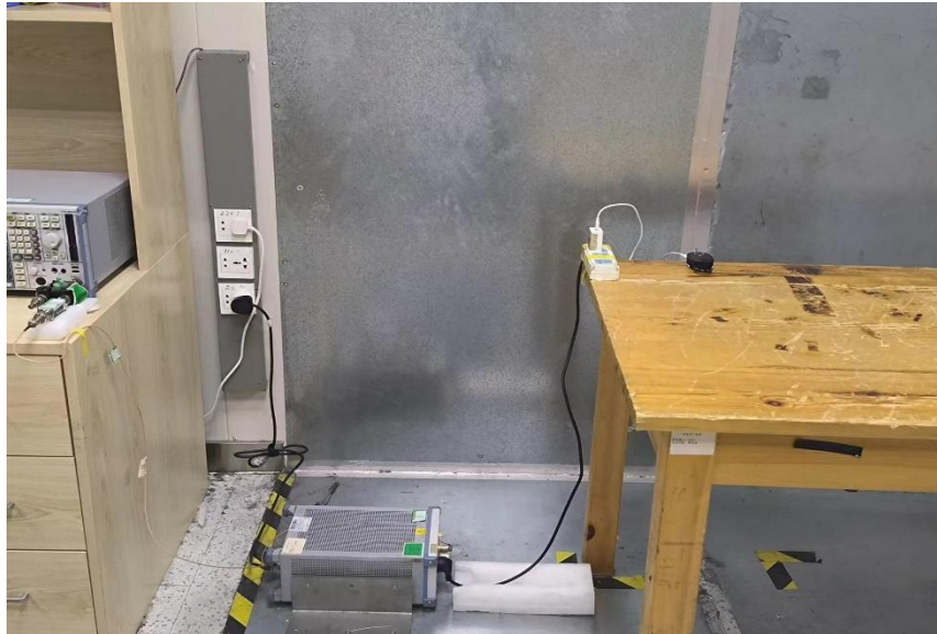
Conducted Emissions
